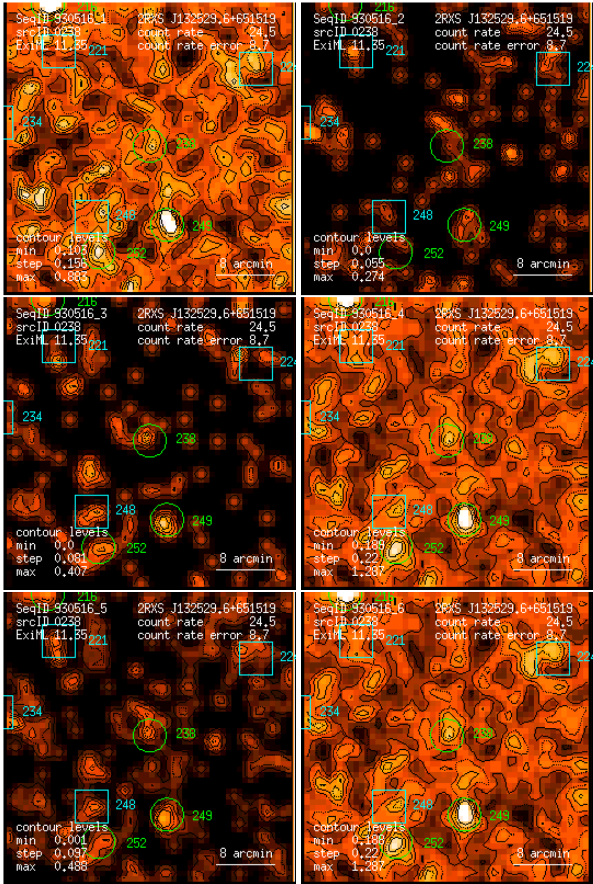
Figure 238: RASS 930516: detection 0238: band rate images, Gaussian filter: (1) PSPC channels 11 – 41, (2) 52 – 90, (3) 91 – 201, (4) 11 – 235, (5) 52 – 201, (6) 11 – 201. Broad band rates in counts/ks. Band rate contour levels in counts/ks/arcmin 2 .
