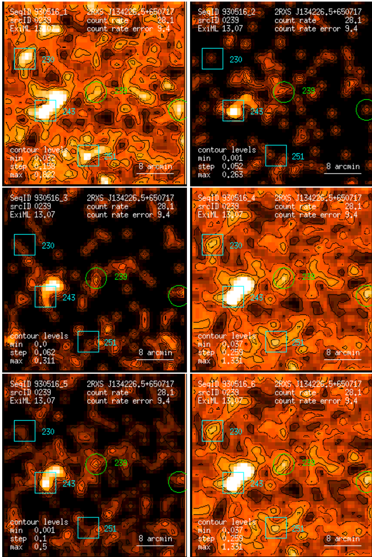
Figure 239: RASS 930516: detection 0239: band rate images, Gaussian filter: (1) PSPC channels 11 – 41, (2) 52 – 90, (3) 91 – 201, (4) 11 – 235, (5) 52 – 201, (6) 11 – 201. Broad band rates in counts/ks. Band rate contour levels in counts/ks/arcmin 2 .
