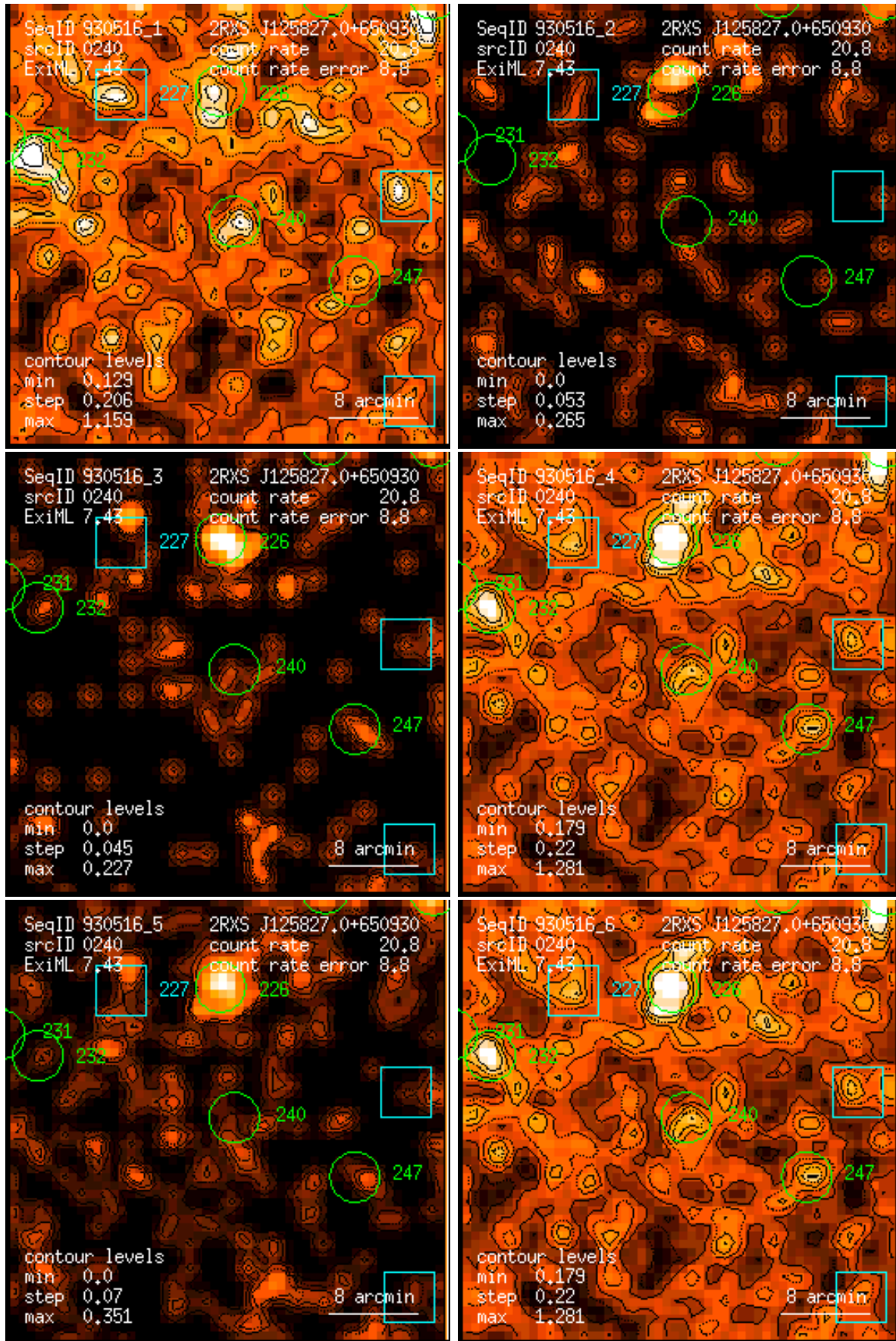
Figure 240: RASS 930516: detection 0240: band rate images, Gaussian filter: (1) PSPC channels 11 – 41, (2) 52 – 90, (3) 91 – 201, (4) 11 – 235, (5) 52 – 201, (6) 11 – 201. Broad band rates in counts/ks. Band rate contour levels in counts/ks/arcmin 2 .
