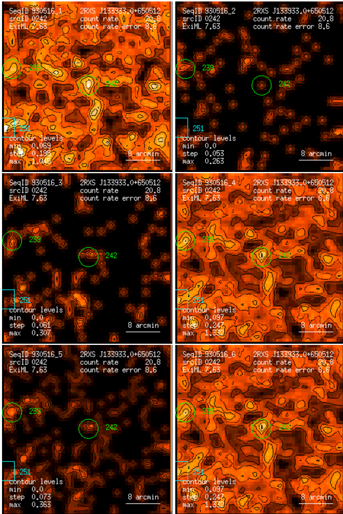
Figure 242: RASS 930516: detection 0242: band rate images, Gaussian filter: (1) PSPC channels 11 – 41, (2) 52 – 90, (3) 91 – 201, (4) 11 – 235, (5) 52 – 201, (6) 11 – 201. Broad band rates in counts/ks. Band rate contour levels in counts/ks/arcmin 2 .
