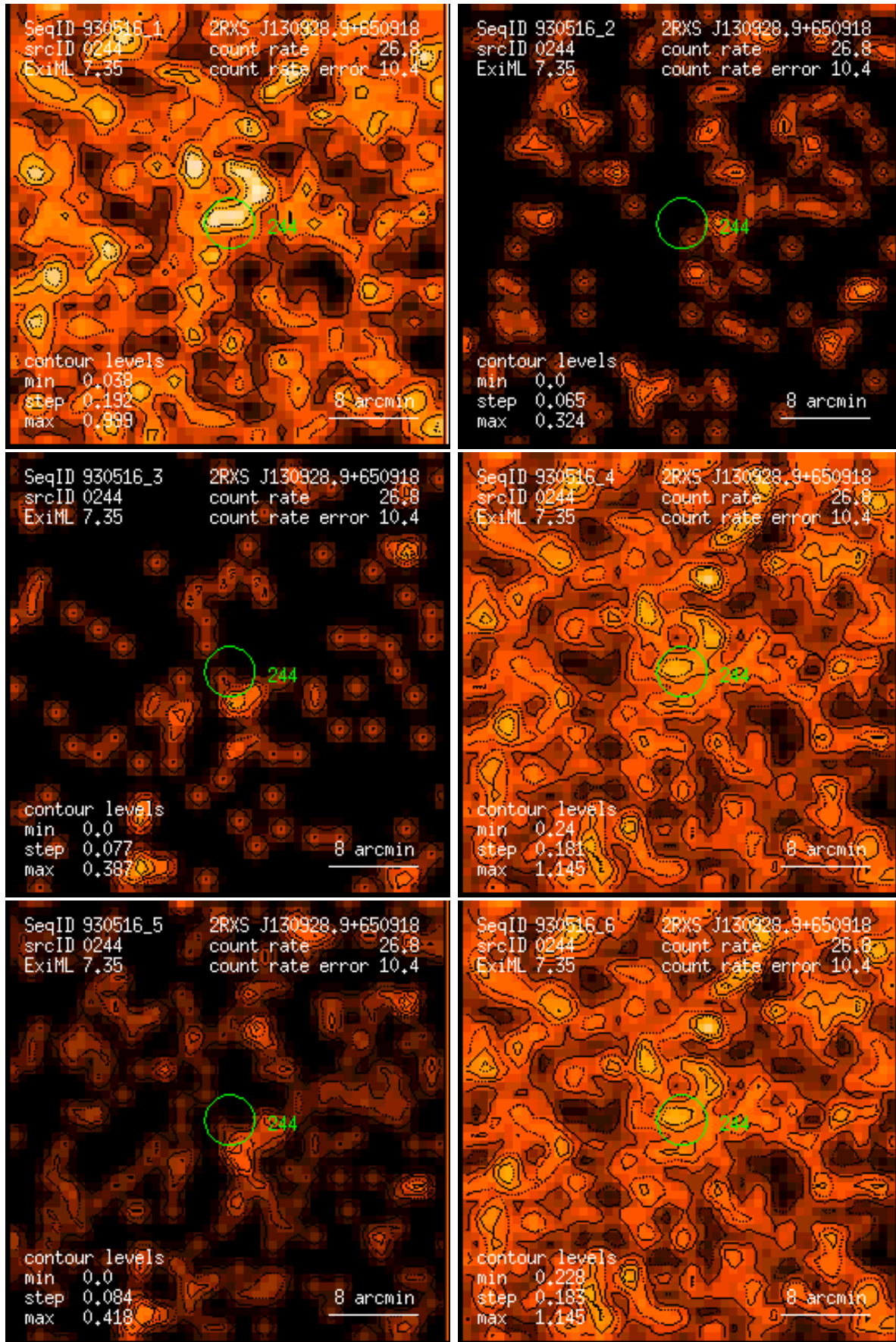
Figure 244: RASS 930516: detection 0244: band rate images, Gaussian filter: (1) PSPC channels 11 – 41, (2) 52 – 90, (3) 91 – 201, (4) 11 – 235, (5) 52 – 201, (6) 11 – 201. Broad band rates in counts/ks. Band rate contour levels in counts/ks/arcmin 2 .
