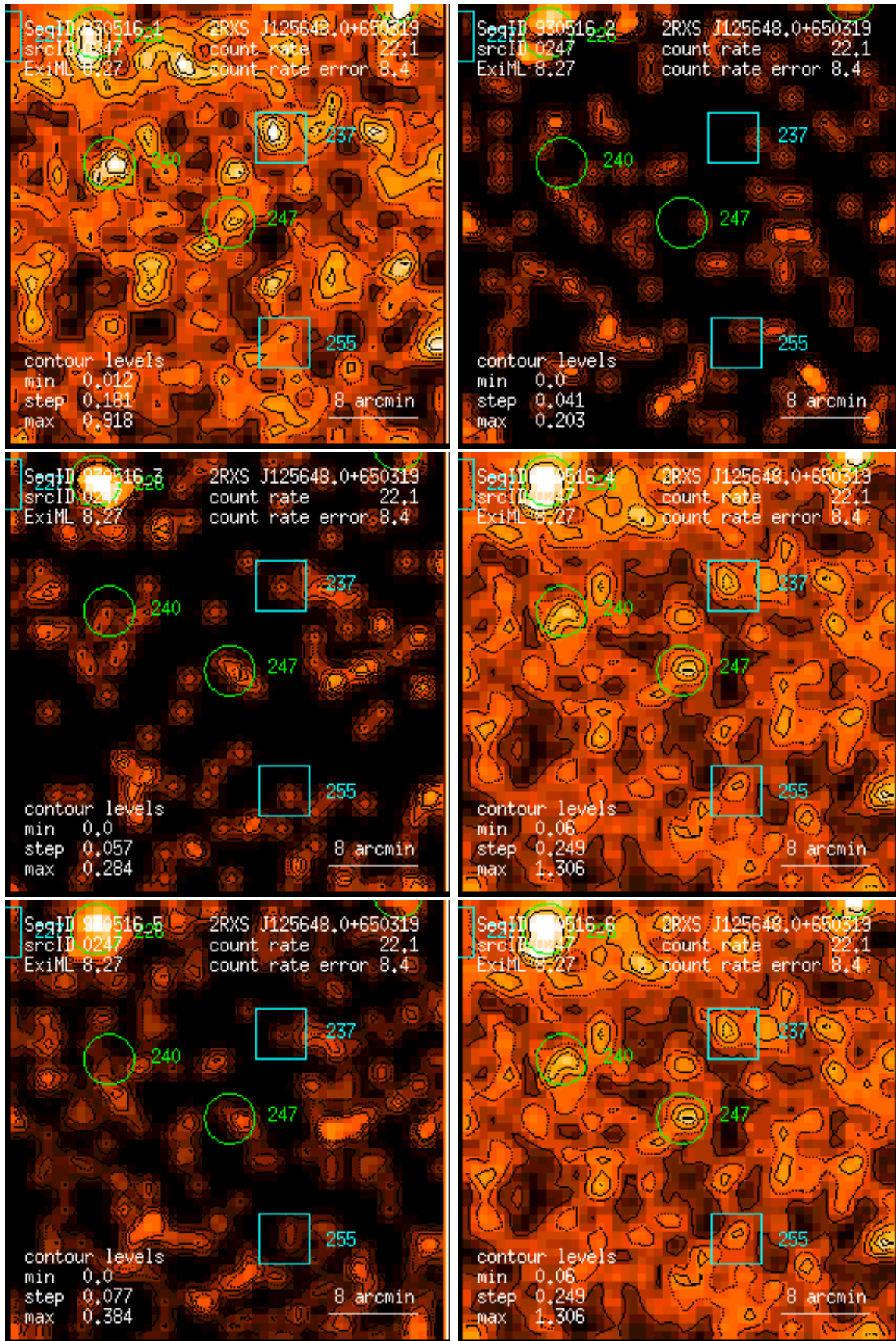
Figure 247: RASS 930516: detection 0247: band rate images, Gaussian filter: (1) PSPC channels 11 – 41, (2) 52 – 90, (3) 91 – 201, (4) 11 – 235, (5) 52 – 201, (6) 11 – 201. Broad band rates in counts/ks. Band rate contour levels in counts/ks/arcmin 2 .
