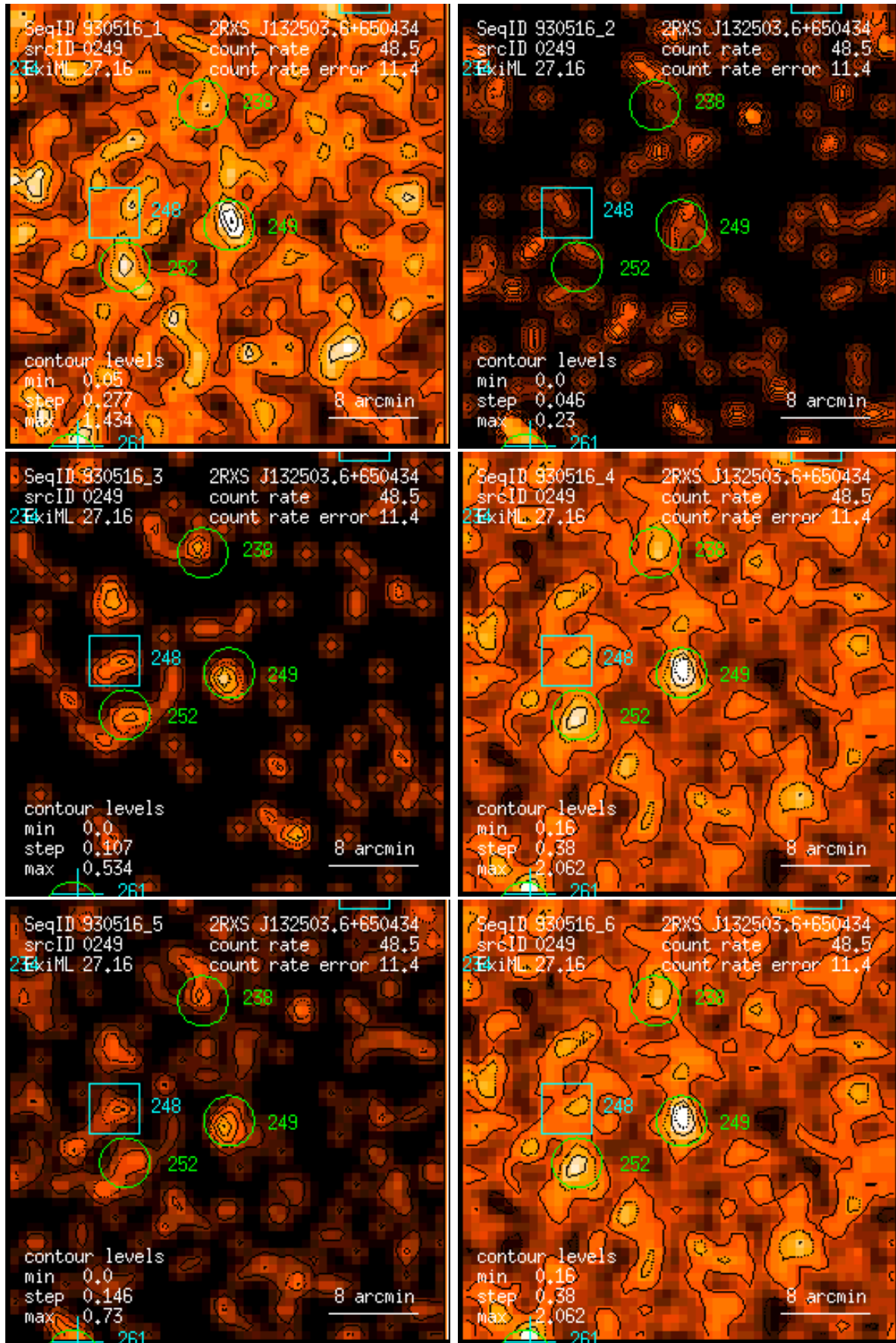
Figure 249: RASS 930516: detection 0249: band rate images, Gaussian filter: (1) PSPC channels 11 – 41, (2) 52 – 90, (3) 91 – 201, (4) 11 – 235, (5) 52 – 201, (6) 11 – 201. Broad band rates in counts/ks. Band rate contour levels in counts/ks/arcmin 2 .
