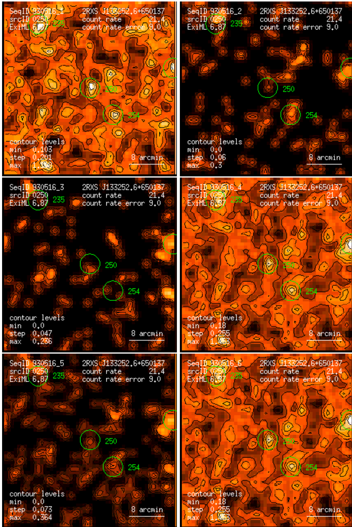
Figure 250: RASS 930516: detection 0250: band rate images, Gaussian filter: (1) PSPC channels 11 – 41, (2) 52 – 90, (3) 91 – 201, (4) 11 – 235, (5) 52 – 201, (6) 11 – 201. Broad band rates in counts/ks. Band rate contour levels in counts/ks/arcmin 2 .
