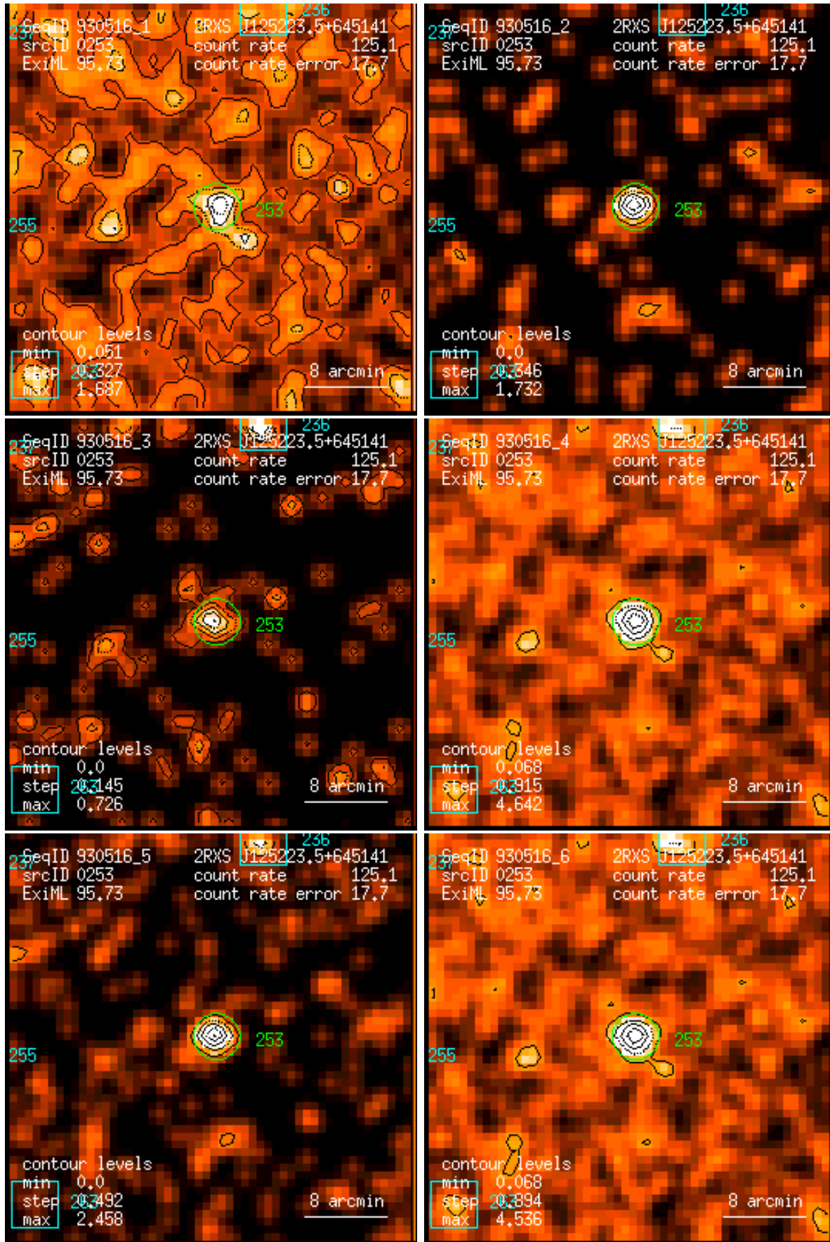
Figure 253: RASS 930516: detection 0253: band rate images, Gaussian filter: (1) PSPC channels 11 – 41, (2) 52 – 90, (3) 91 – 201, (4) 11 – 235, (5) 52 – 201, (6) 11 – 201. Broad band rates in counts/ks. Band rate contour levels in counts/ks/arcmin 2 .
