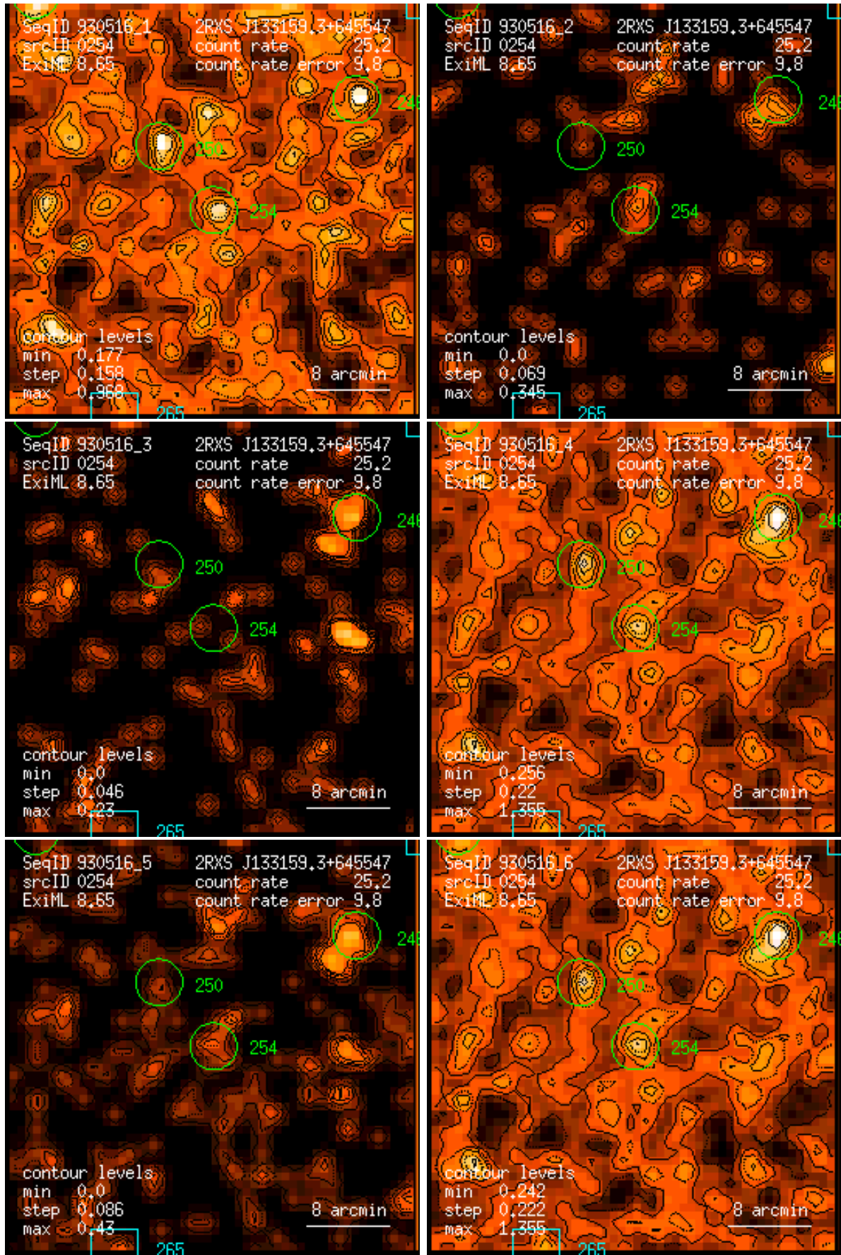
Figure 254: RASS 930516: detection 0254: band rate images, Gaussian filter: (1) PSPC channels 11 – 41, (2) 52 – 90, (3) 91 – 201, (4) 11 – 235, (5) 52 – 201, (6) 11 – 201. Broad band rates in counts/ks. Band rate contour levels in counts/ks/arcmin 2 .
