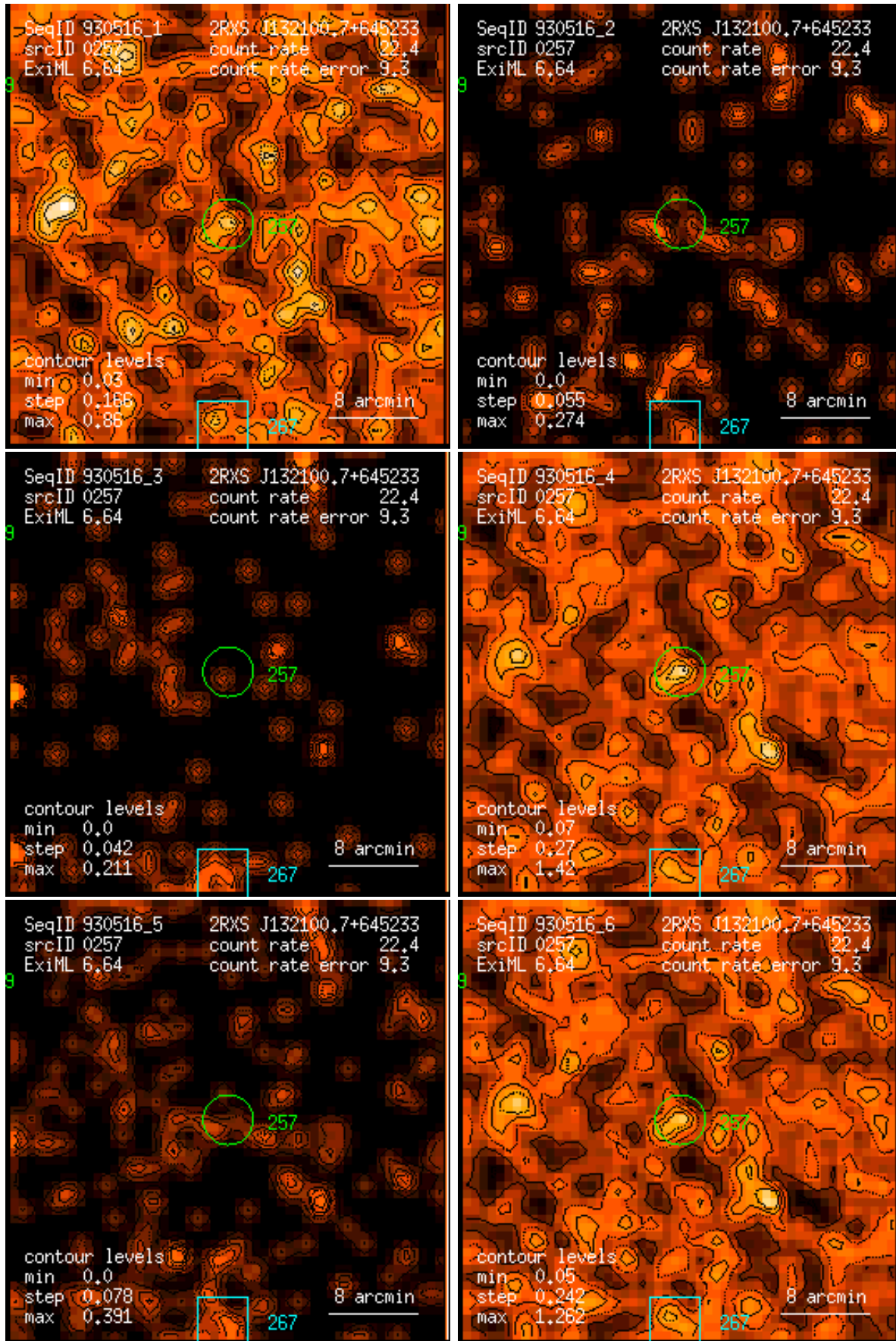
Figure 257: RASS 930516: detection 0257: band rate images, Gaussian filter: (1) PSPC channels 11 – 41, (2) 52 – 90, (3) 91 – 201, (4) 11 – 235, (5) 52 – 201, (6) 11 – 201. Broad band rates in counts/ks. Band rate contour levels in counts/ks/arcmin 2 .
