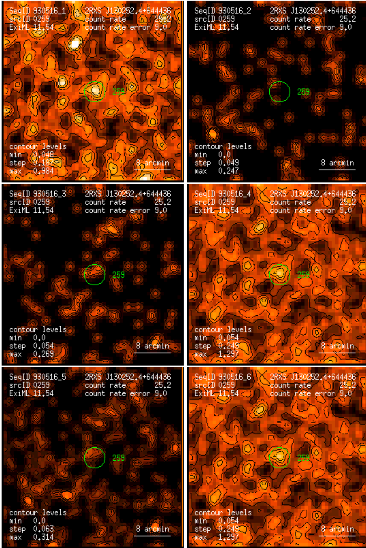
Figure 259: RASS 930516: detection 0259: band rate images, Gaussian filter: (1) PSPC channels 11 – 41, (2) 52 – 90, (3) 91 – 201, (4) 11 – 235, (5) 52 – 201, (6) 11 – 201. Broad band rates in counts/ks. Band rate contour levels in counts/ks/arcmin 2 .
