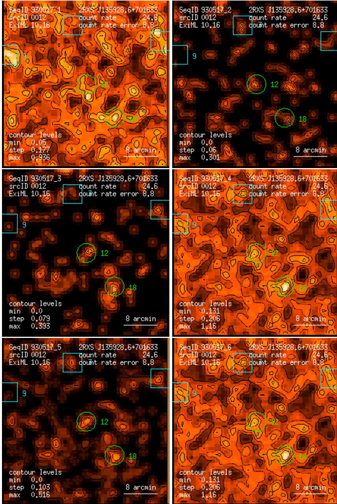
Figure 12: RASS 930517: detection 0012: band rate images, Gaussian filter: (1) PSPC channels 11 – 41, (2) 52 – 90, (3) 91 – 201, (4) 11 – 235, (5) 52 – 201, (6) 11 – 201. Broad band rates in counts/ks. Band rate contour levels in counts/ks/arcmin 2 .
