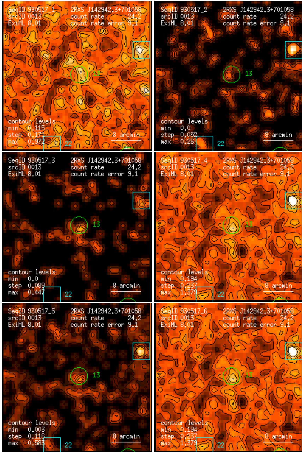
Figure 13: RASS 930517: detection 0013: band rate images, Gaussian filter: (1) PSPC channels 11 – 41, (2) 52 – 90, (3) 91 – 201, (4) 11 – 235, (5) 52 – 201, (6) 11 – 201. Broad band rates in counts/ks. Band rate contour levels in counts/ks/arcmin 2 .
