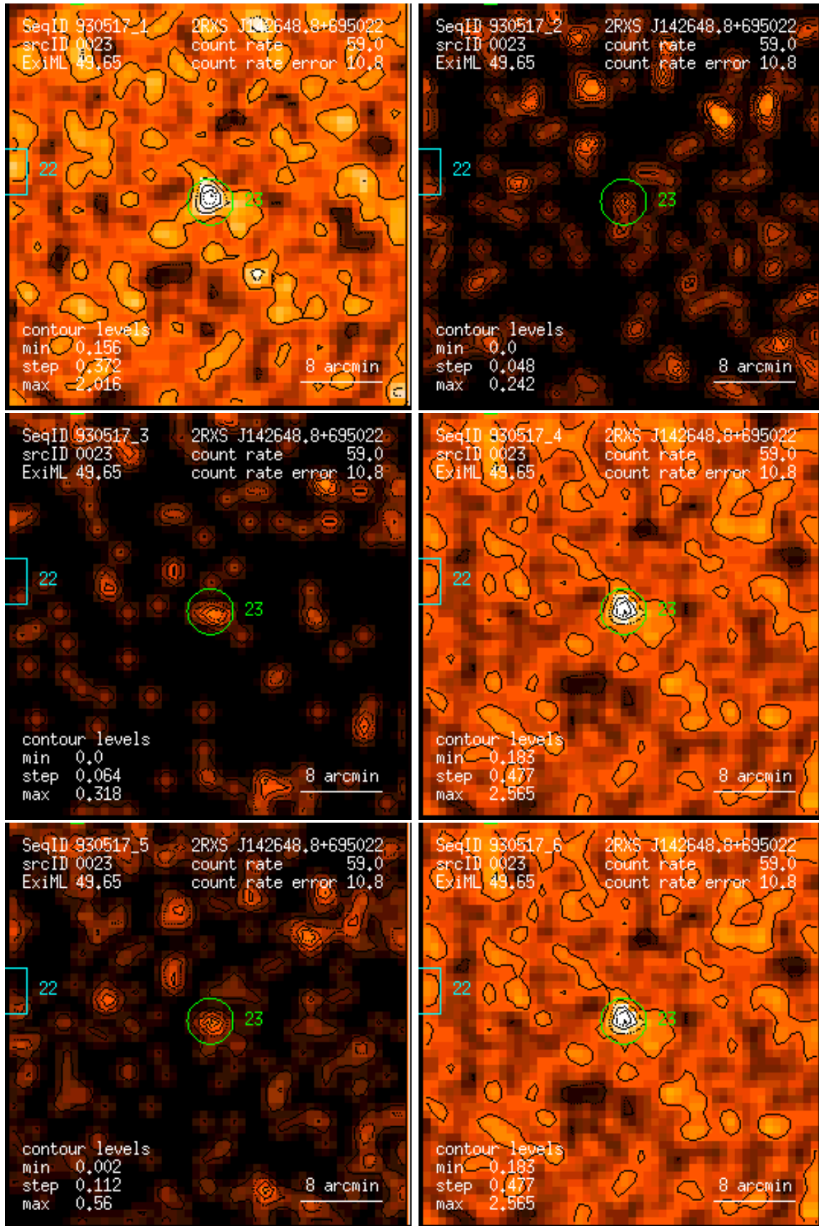
Figure 23: RASS 930517: detection 0023: band rate images, Gaussian filter: (1) PSPC channels 11 – 41, (2) 52 – 90, (3) 91 – 201, (4) 11 – 235, (5) 52 – 201, (6) 11 – 201. Broad band rates in counts/ks. Band rate contour levels in counts/ks/arcmin 2 .
