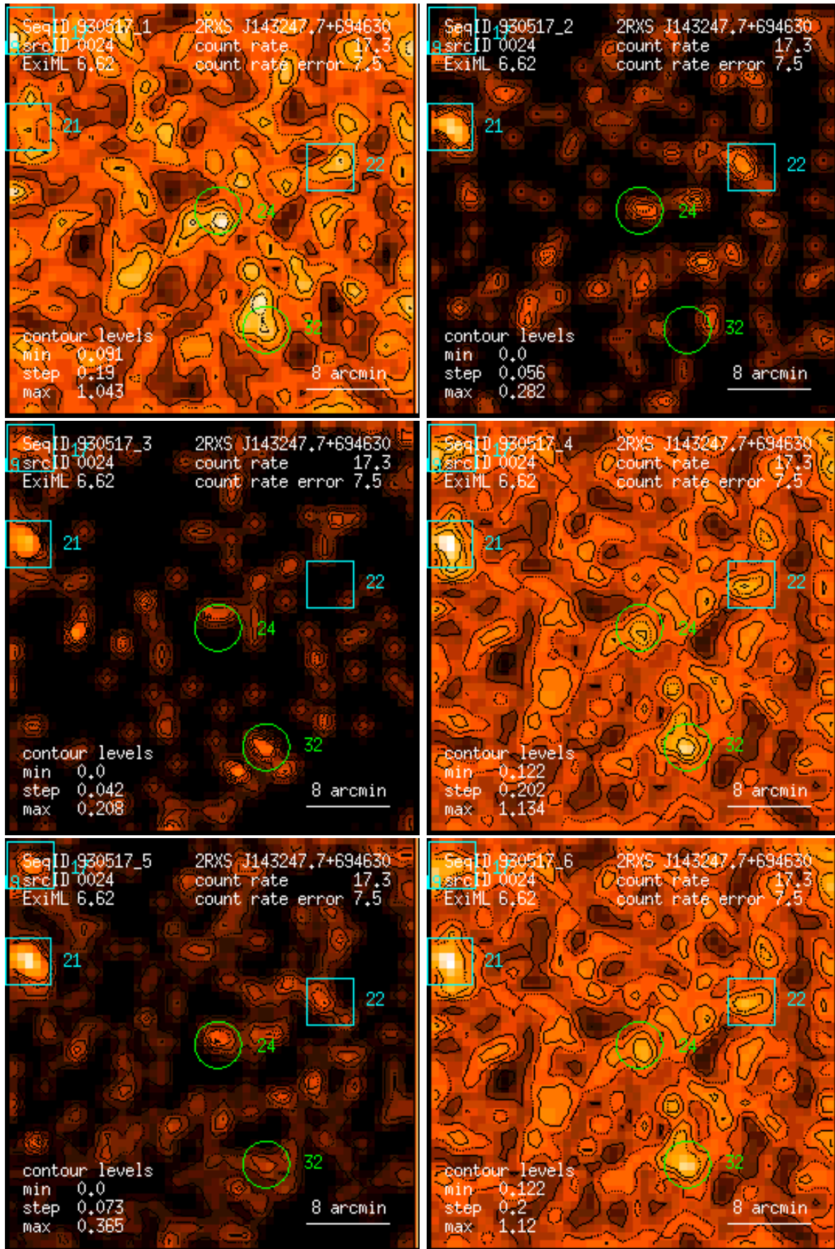
Figure 24: RASS 930517: detection 0024: band rate images, Gaussian filter: (1) PSPC channels 11 – 41, (2) 52 – 90, (3) 91 – 201, (4) 11 – 235, (5) 52 – 201, (6) 11 – 201. Broad band rates in counts/ks. Band rate contour levels in counts/ks/arcmin 2 .
