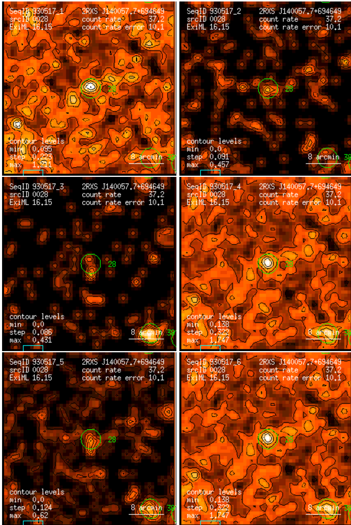
Figure 28: RASS 930517: detection 0028: band rate images, Gaussian filter: (1) PSPC channels 11 – 41, (2) 52 – 90, (3) 91 – 201, (4) 11 – 235, (5) 52 – 201, (6) 11 – 201. Broad band rates in counts/ks. Band rate contour levels in counts/ks/arcmin 2 .
