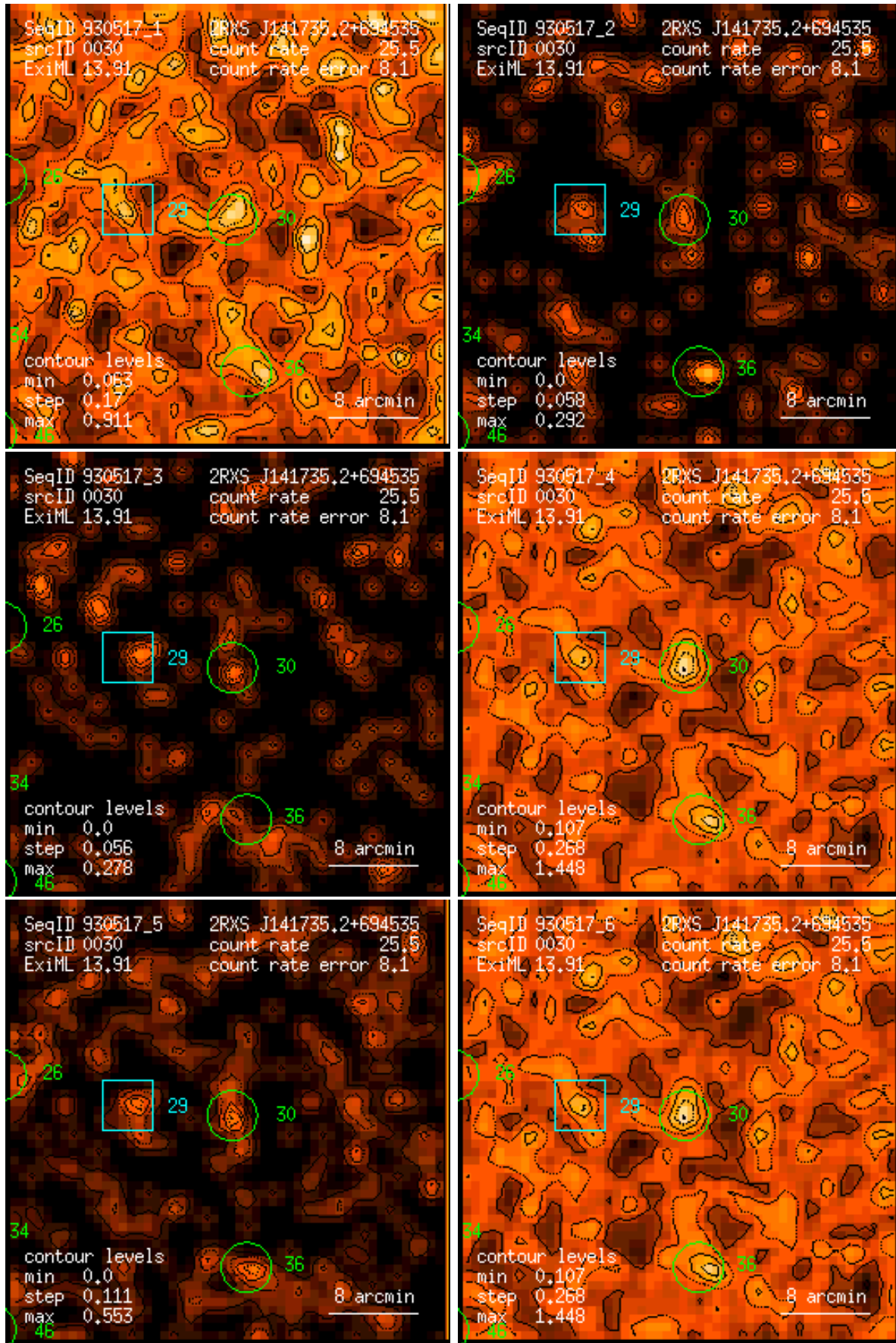
Figure 30: RASS 930517: detection 0030: band rate images, Gaussian filter: (1) PSPC channels 11 – 41, (2) 52 – 90, (3) 91 – 201, (4) 11 – 235, (5) 52 – 201, (6) 11 – 201. Broad band rates in counts/ks. Band rate contour levels in counts/ks/arcmin 2 .
