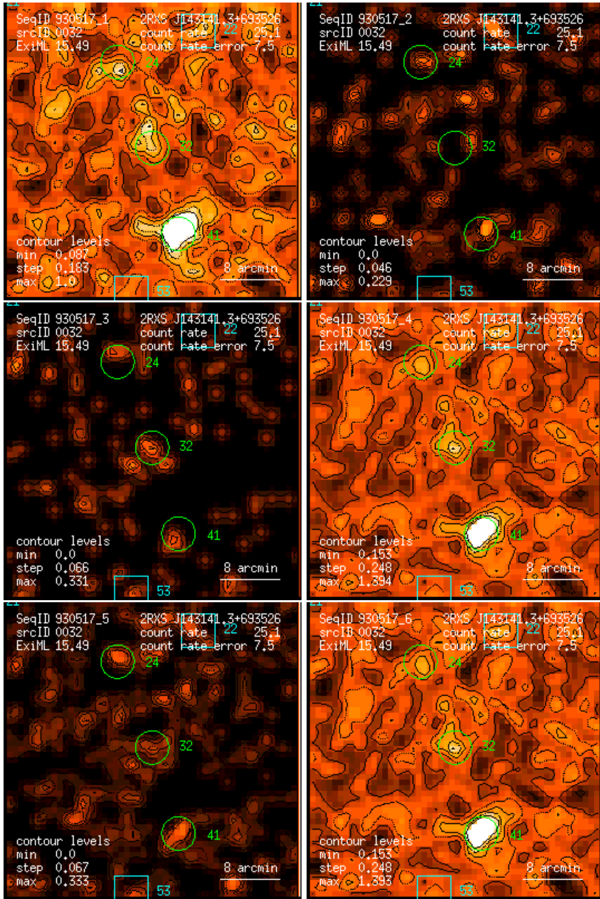
Figure 32: RASS 930517: detection 0032: band rate images, Gaussian filter: (1) PSPC channels 11 – 41, (2) 52 – 90, (3) 91 – 201, (4) 11 – 235, (5) 52 – 201, (6) 11 – 201. Broad band rates in counts/ks. Band rate contour levels in counts/ks/arcmin 2 .
