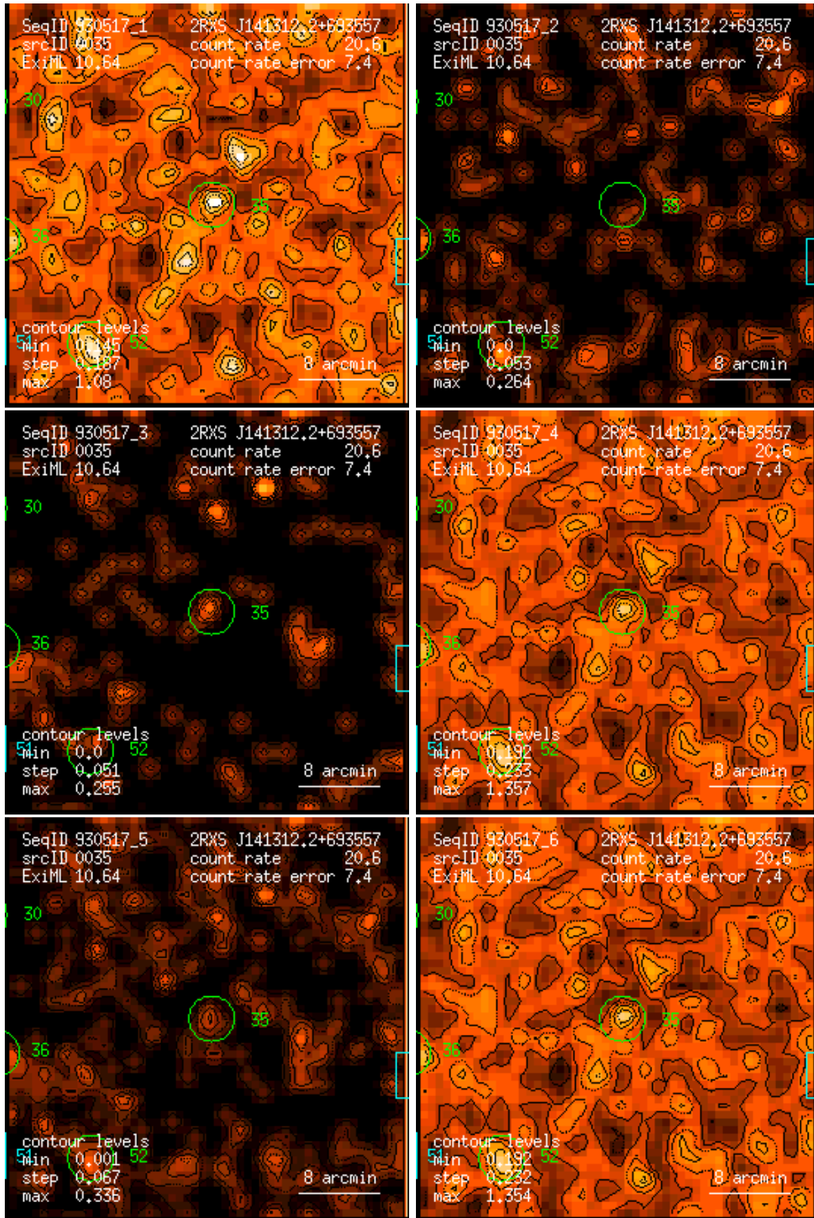
Figure 35: RASS 930517: detection 0035: band rate images, Gaussian filter: (1) PSPC channels 11 – 41, (2) 52 – 90, (3) 91 – 201, (4) 11 – 235, (5) 52 – 201, (6) 11 – 201. Broad band rates in counts/ks. Band rate contour levels in counts/ks/arcmin 2 .
