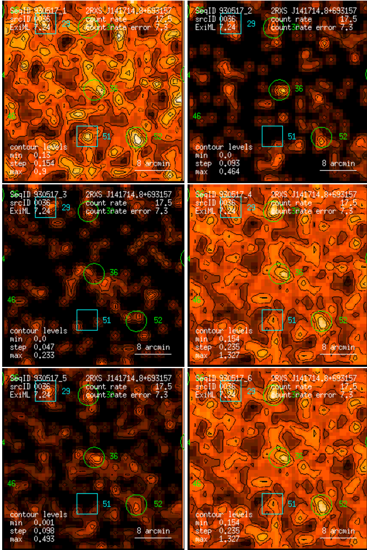
Figure 36: RASS 930517: detection 0036: band rate images, Gaussian filter: (1) PSPC channels 11 – 41, (2) 52 – 90, (3) 91 – 201, (4) 11 – 235, (5) 52 – 201, (6) 11 – 201. Broad band rates in counts/ks. Band rate contour levels in counts/ks/arcmin 2 .
