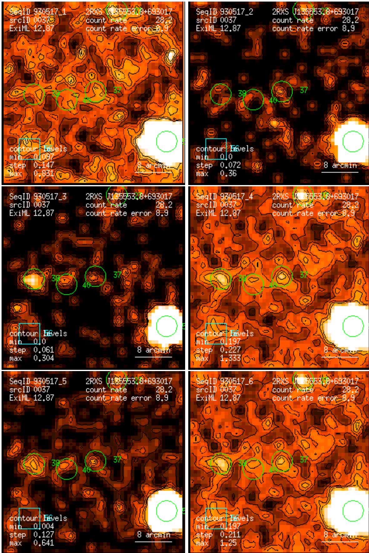
Figure 37: RASS 930517: detection 0037: band rate images, Gaussian filter: (1) PSPC channels 11 – 41, (2) 52 – 90, (3) 91 – 201, (4) 11 – 235, (5) 52 – 201, (6) 11 – 201. Broad band rates in counts/ks. Band rate contour levels in counts/ks/arcmin 2 .
