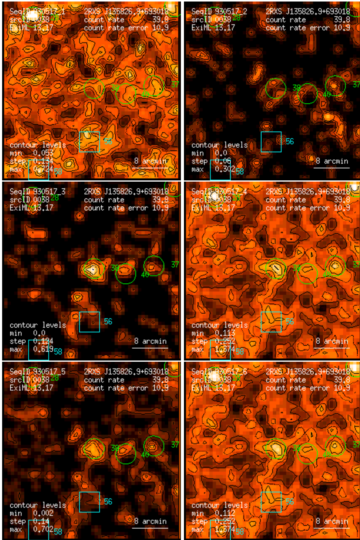
Figure 38: RASS 930517: detection 0038: band rate images, Gaussian filter: (1) PSPC channels 11 – 41, (2) 52 – 90, (3) 91 – 201, (4) 11 – 235, (5) 52 – 201, (6) 11 – 201. Broad band rates in counts/ks. Band rate contour levels in counts/ks/arcmin 2 .
