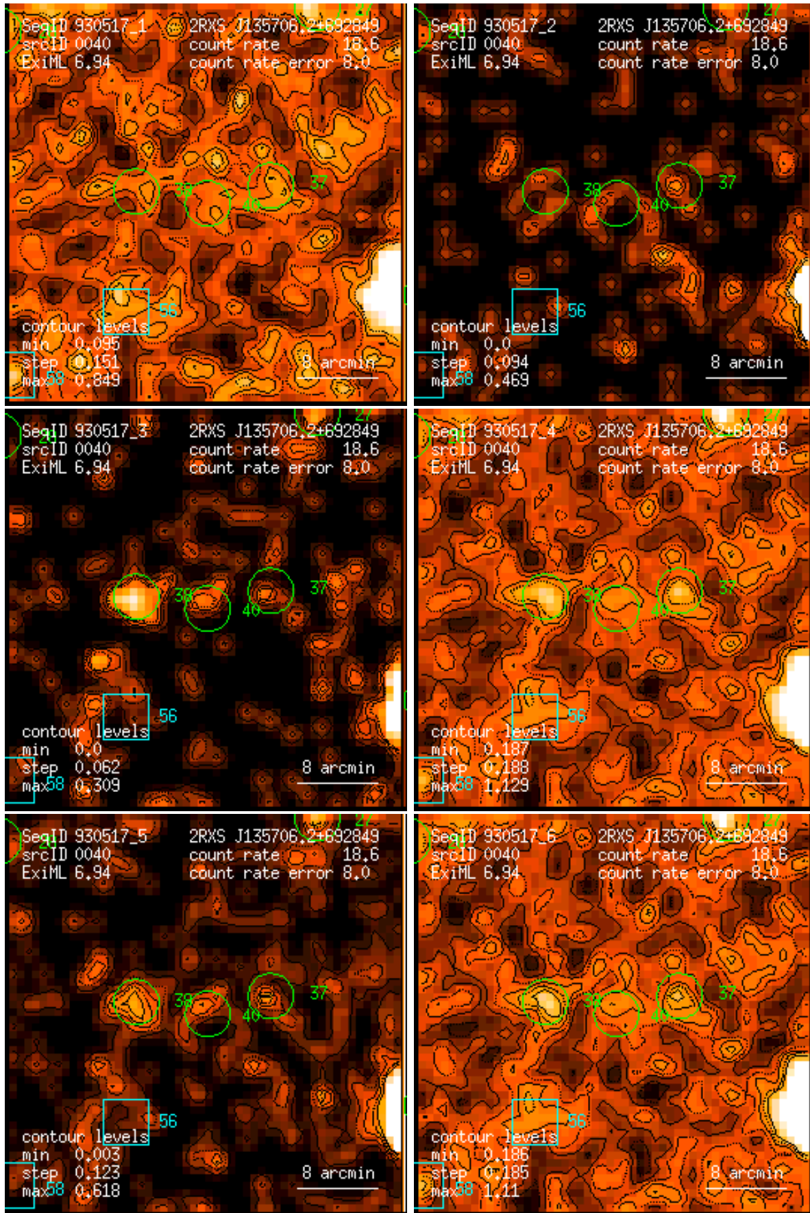
Figure 40: RASS 930517: detection 0040: band rate images, Gaussian filter: (1) PSPC channels 11 – 41, (2) 52 – 90, (3) 91 – 201, (4) 11 – 235, (5) 52 – 201, (6) 11 – 201. Broad band rates in counts/ks. Band rate contour levels in counts/ks/arcmin 2 .
