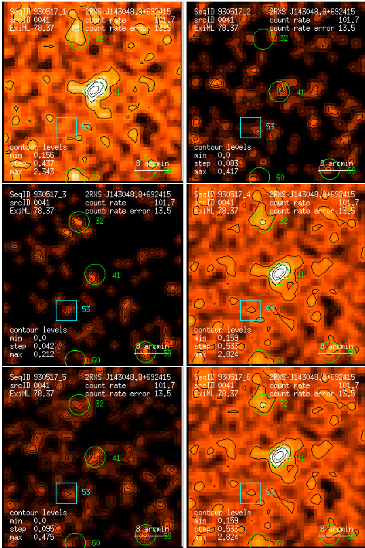
Figure 41: RASS 930517: detection 0041: band rate images, Gaussian filter: (1) PSPC channels 11 – 41, (2) 52 – 90, (3) 91 – 201, (4) 11 – 235, (5) 52 – 201, (6) 11 – 201. Broad band rates in counts/ks. Band rate contour levels in counts/ks/arcmin 2 .
