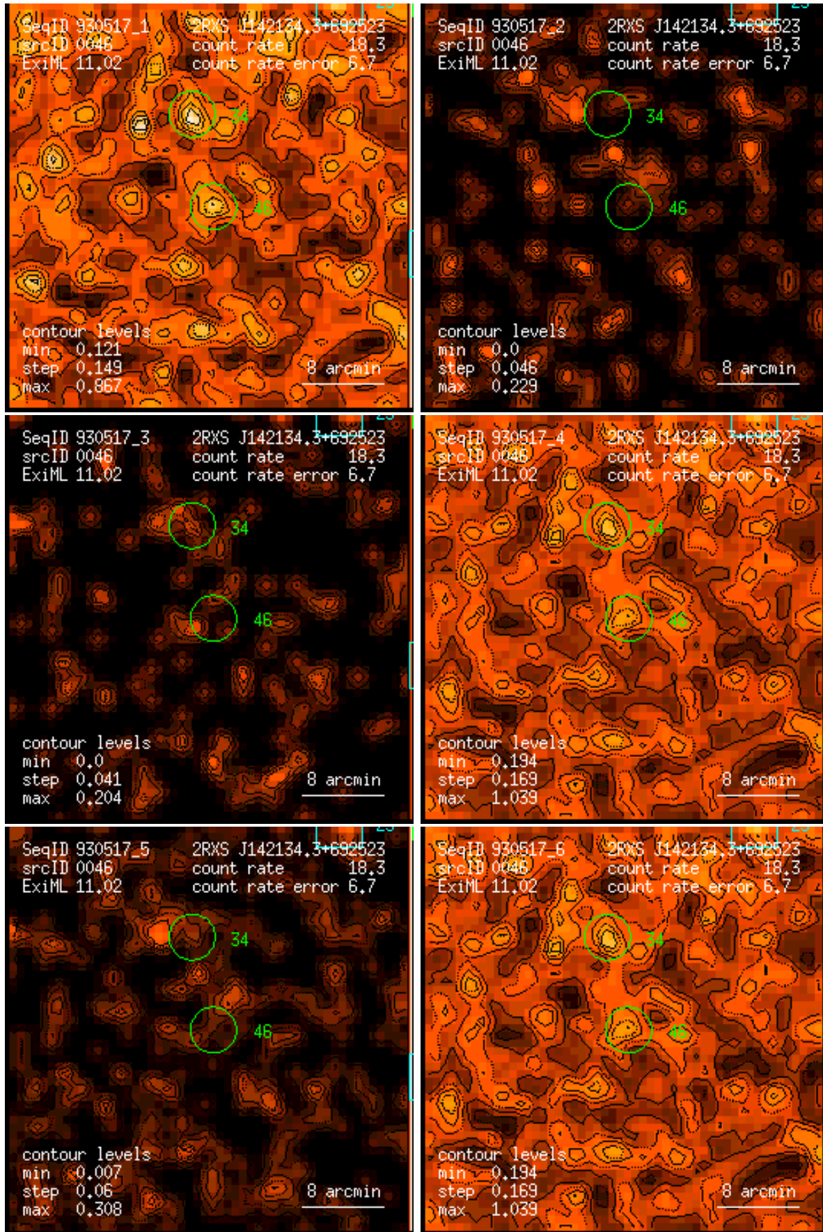
Figure 46: RASS 930517: detection 0046: band rate images, Gaussian filter: (1) PSPC channels 11 – 41, (2) 52 – 90, (3) 91 – 201, (4) 11 – 235, (5) 52 – 201, (6) 11 – 201. Broad band rates in counts/ks. Band rate contour levels in counts/ks/arcmin 2 .
