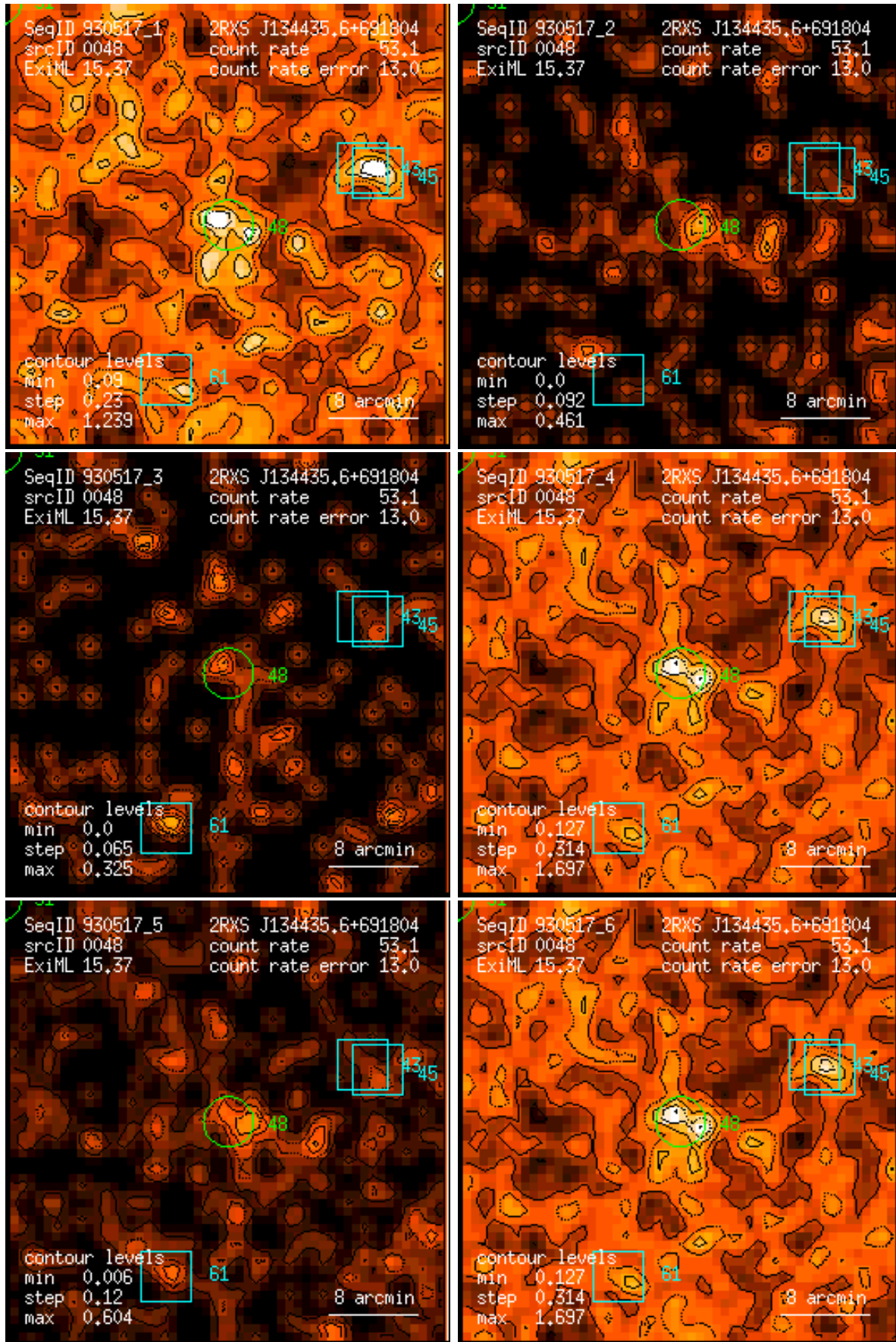
Figure 48: RASS 930517: detection 0048: band rate images, Gaussian filter: (1) PSPC channels 11 – 41, (2) 52 – 90, (3) 91 – 201, (4) 11 – 235, (5) 52 – 201, (6) 11 – 201. Broad band rates in counts/ks. Band rate contour levels in counts/ks/arcmin 2 .
