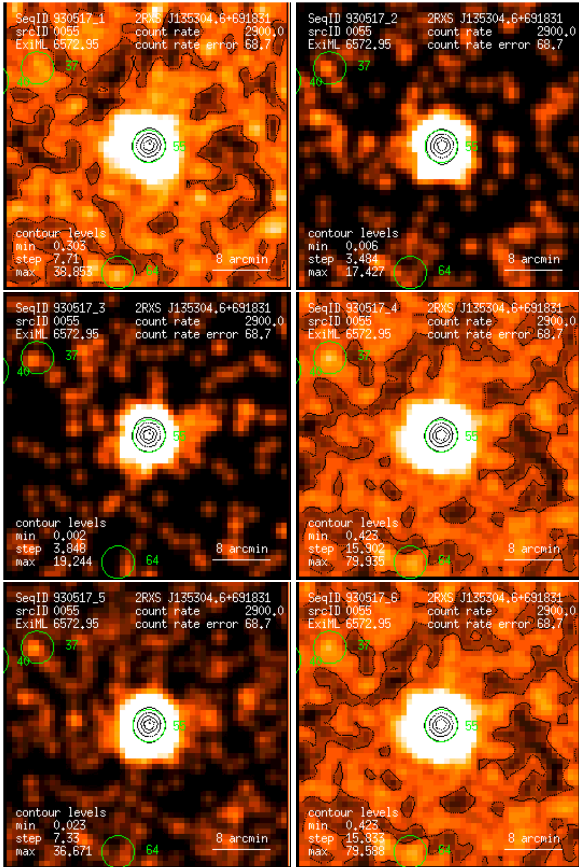
Figure 55: RASS 930517: detection 0055: band rate images, Gaussian filter: (1) PSPC channels 11 – 41, (2) 52 – 90, (3) 91 – 201, (4) 11 – 235, (5) 52 – 201, (6) 11 – 201. Broad band rates in counts/ks. Band rate contour levels in counts/ks/arcmin 2 .
