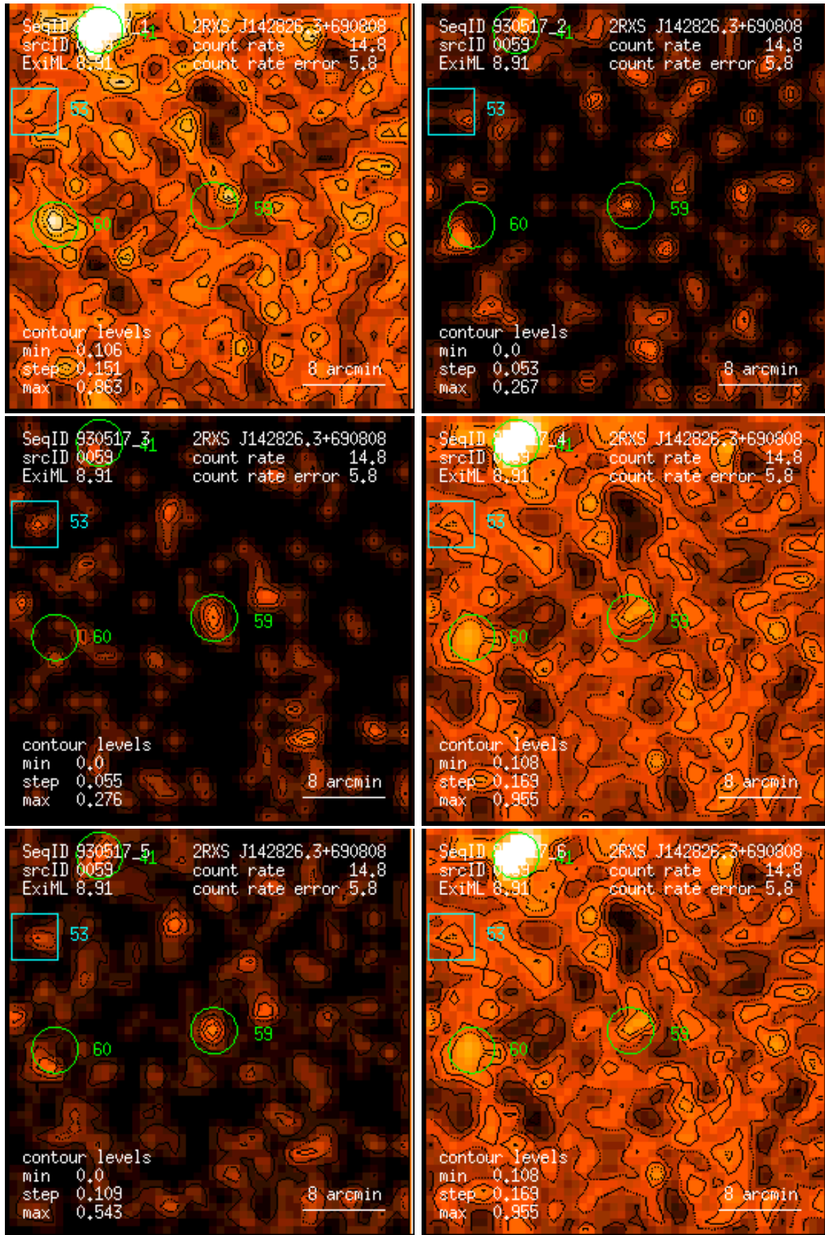
Figure 59: RASS 930517: detection 0059: band rate images, Gaussian filter: (1) PSPC channels 11 – 41, (2) 52 – 90, (3) 91 – 201, (4) 11 – 235, (5) 52 – 201, (6) 11 – 201. Broad band rates in counts/ks. Band rate contour levels in counts/ks/arcmin 2 .
