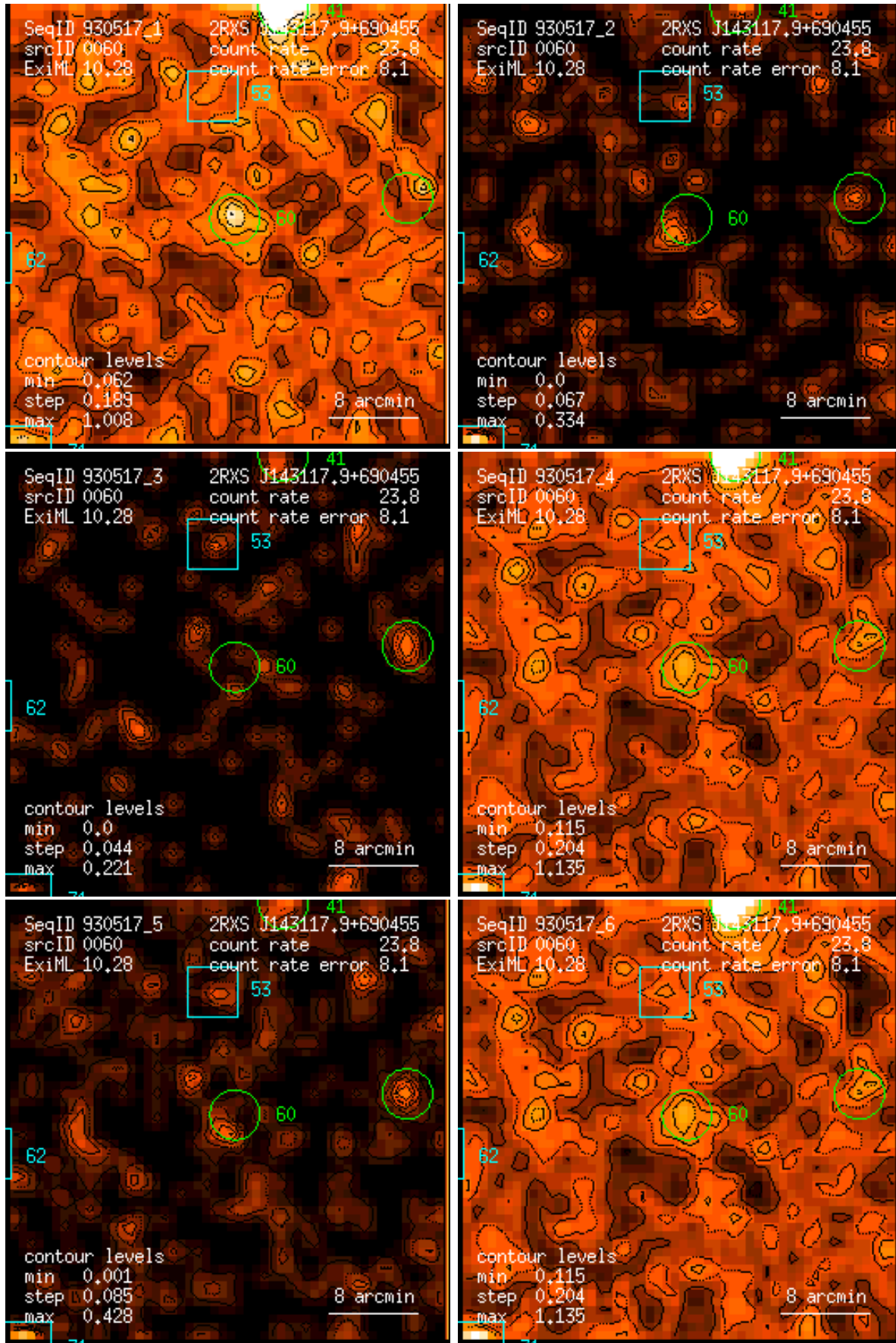
Figure 60: RASS 930517: detection 0060: band rate images, Gaussian filter: (1) PSPC channels 11 – 41, (2) 52 – 90, (3) 91 – 201, (4) 11 – 235, (5) 52 – 201, (6) 11 – 201. Broad band rates in counts/ks. Band rate contour levels in counts/ks/arcmin 2 .
