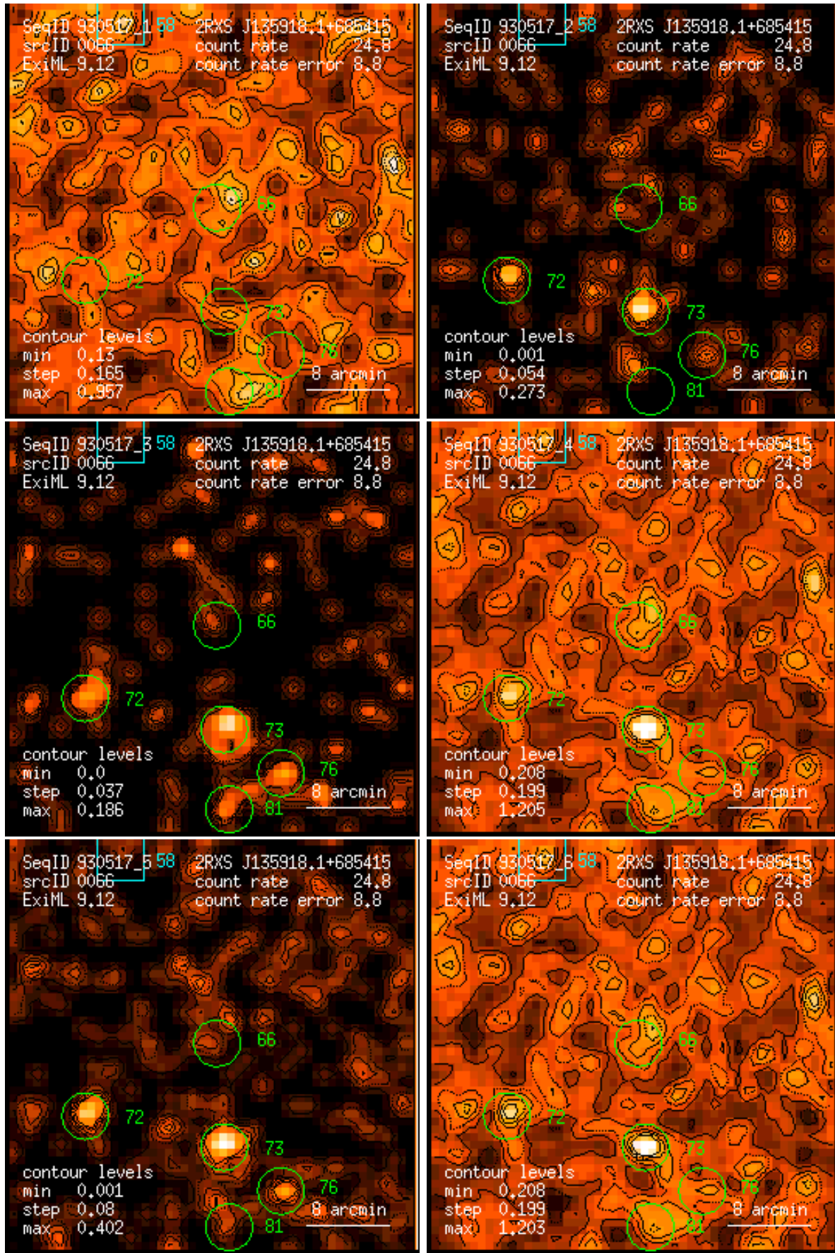
Figure 66: RASS 930517: detection 0066: band rate images, Gaussian filter: (1) PSPC channels 11 – 41, (2) 52 – 90, (3) 91 – 201, (4) 11 – 235, (5) 52 – 201, (6) 11 – 201. Broad band rates in counts/ks. Band rate contour levels in counts/ks/arcmin 2 .
