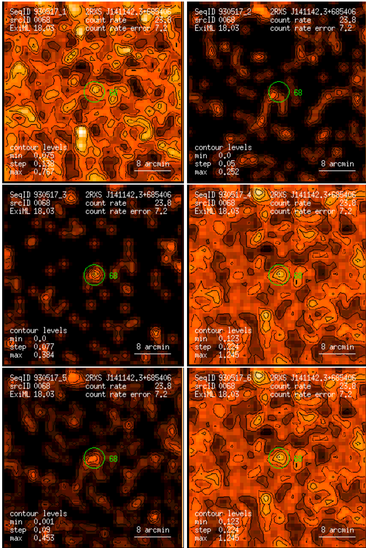
Figure 68: RASS 930517: detection 0068: band rate images, Gaussian filter: (1) PSPC channels 11 – 41, (2) 52 – 90, (3) 91 – 201, (4) 11 – 235, (5) 52 – 201, (6) 11 – 201. Broad band rates in counts/ks. Band rate contour levels in counts/ks/arcmin 2 .
