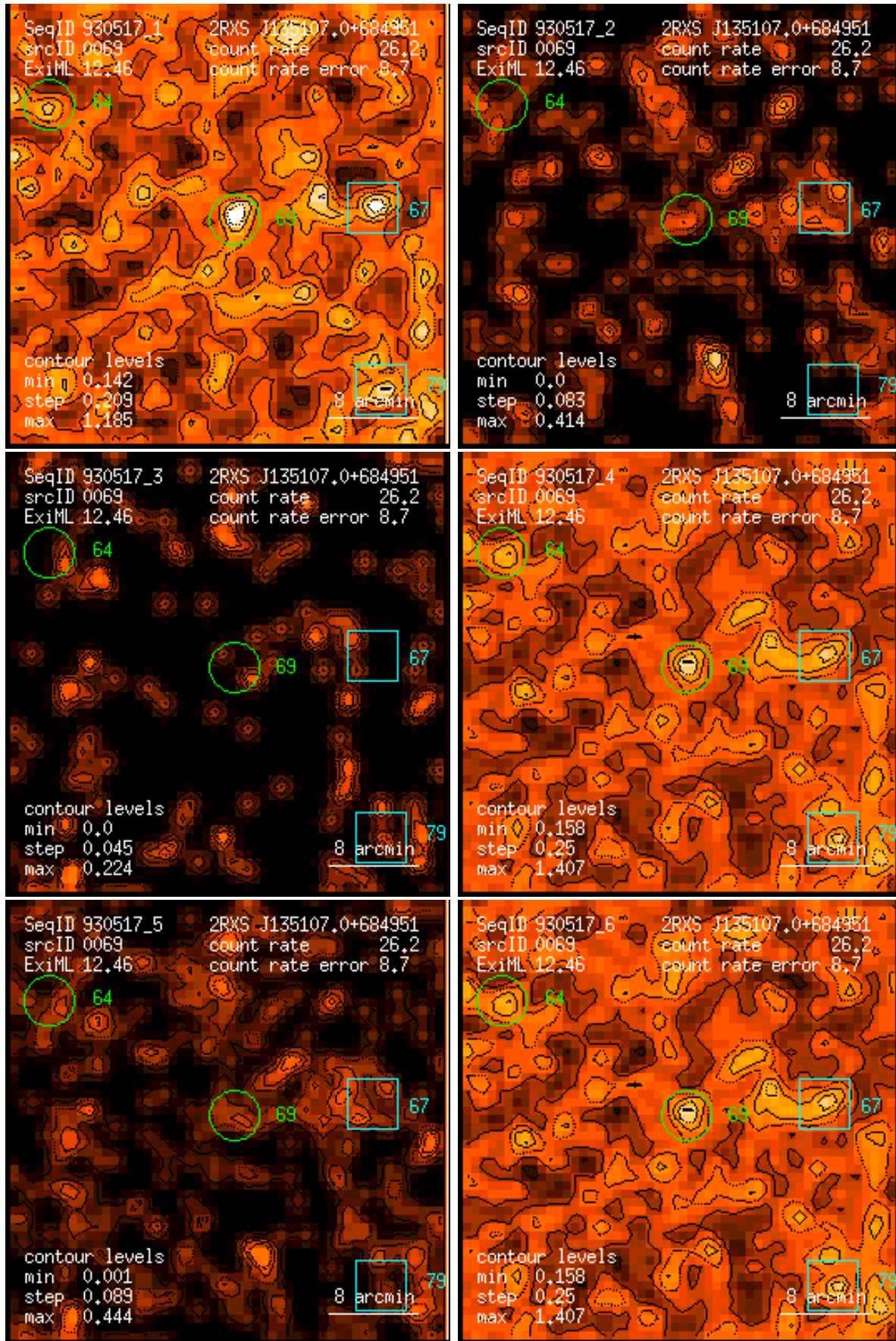
Figure 69: RASS 930517: detection 0069: band rate images, Gaussian filter: (1) PSPC channels 11 – 41, (2) 52 – 90, (3) 91 – 201, (4) 11 – 235, (5) 52 – 201, (6) 11 – 201. Broad band rates in counts/ks. Band rate contour levels in counts/ks/arcmin 2 .
