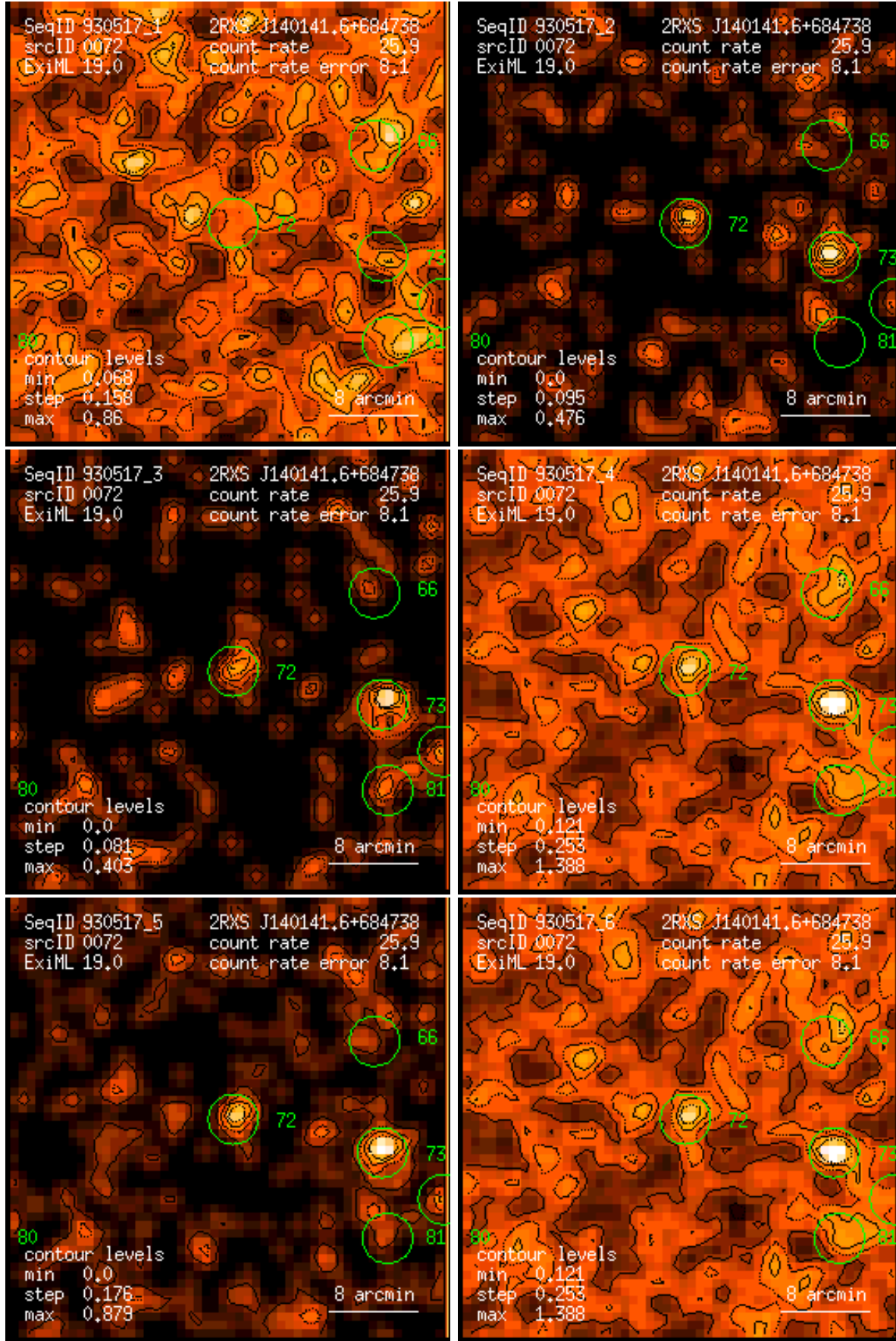
Figure 72: RASS 930517: detection 0072: band rate images, Gaussian filter: (1) PSPC channels 11 – 41, (2) 52 – 90, (3) 91 – 201, (4) 11 – 235, (5) 52 – 201, (6) 11 – 201. Broad band rates in counts/ks. Band rate contour levels in counts/ks/arcmin 2 .
