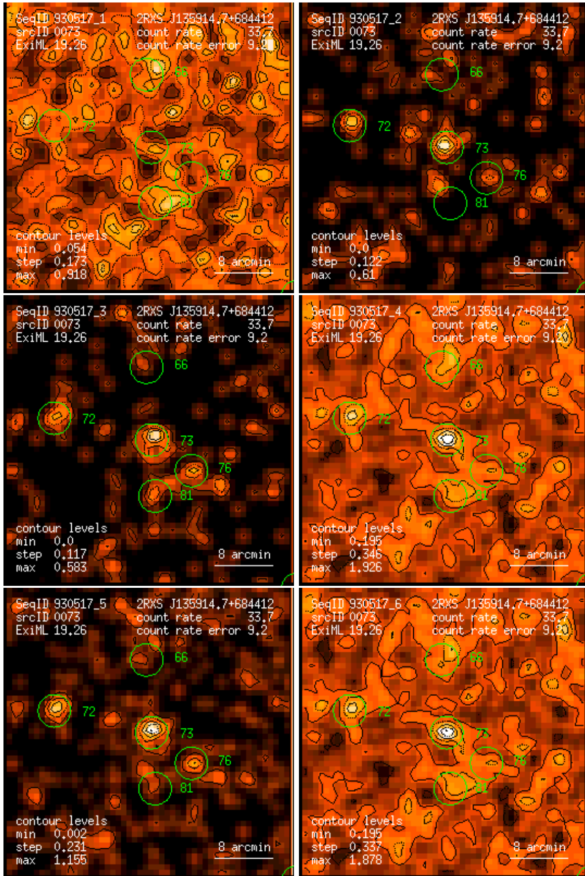
Figure 73: RASS 930517: detection 0073: band rate images, Gaussian filter: (1) PSPC channels 11 – 41, (2) 52 – 90, (3) 91 – 201, (4) 11 – 235, (5) 52 – 201, (6) 11 – 201. Broad band rates in counts/ks. Band rate contour levels in counts/ks/arcmin 2 .
