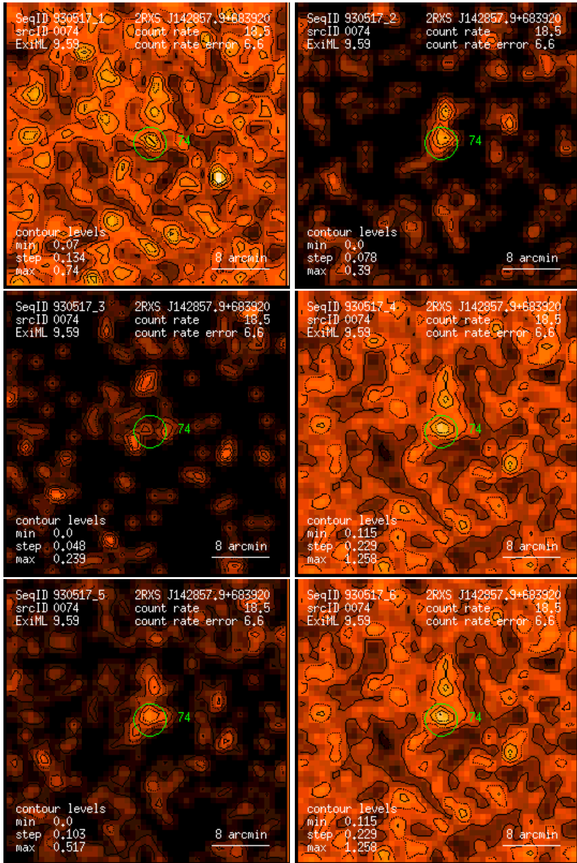
Figure 74: RASS 930517: detection 0074: band rate images, Gaussian filter: (1) PSPC channels 11 – 41, (2) 52 – 90, (3) 91 – 201, (4) 11 – 235, (5) 52 – 201, (6) 11 – 201. Broad band rates in counts/ks. Band rate contour levels in counts/ks/arcmin 2 .
