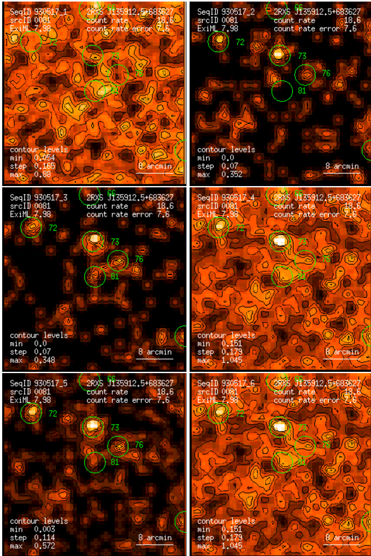
Figure 81: RASS 930517: detection 0081: band rate images, Gaussian filter: (1) PSPC channels 11 – 41, (2) 52 – 90, (3) 91 – 201, (4) 11 – 235, (5) 52 – 201, (6) 11 – 201. Broad band rates in counts/ks. Band rate contour levels in counts/ks/arcmin 2 .
