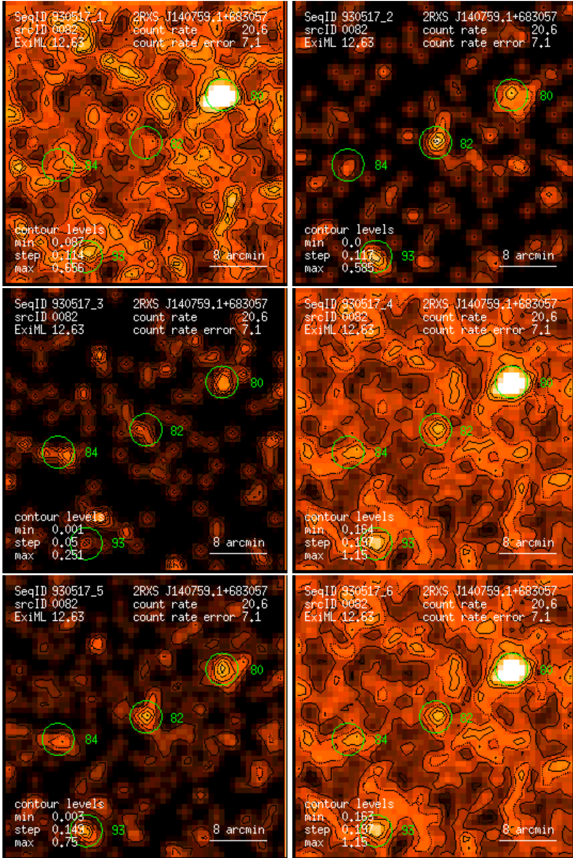
Figure 82: RASS 930517: detection 0082: band rate images, Gaussian filter: (1) PSPC channels 11 – 41, (2) 52 – 90, (3) 91 – 201, (4) 11 – 235, (5) 52 – 201, (6) 11 – 201. Broad band rates in counts/ks. Band rate contour levels in counts/ks/arcmin 2 .
