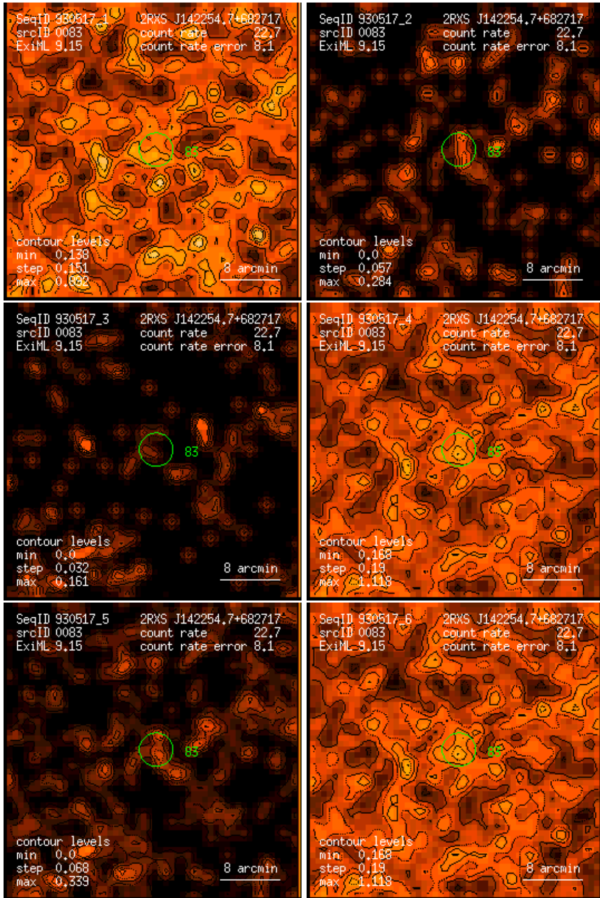
Figure 83: RASS 930517: detection 0083: band rate images, Gaussian filter: (1) PSPC channels 11 – 41, (2) 52 – 90, (3) 91 – 201, (4) 11 – 235, (5) 52 – 201, (6) 11 – 201. Broad band rates in counts/ks. Band rate contour levels in counts/ks/arcmin 2 .
