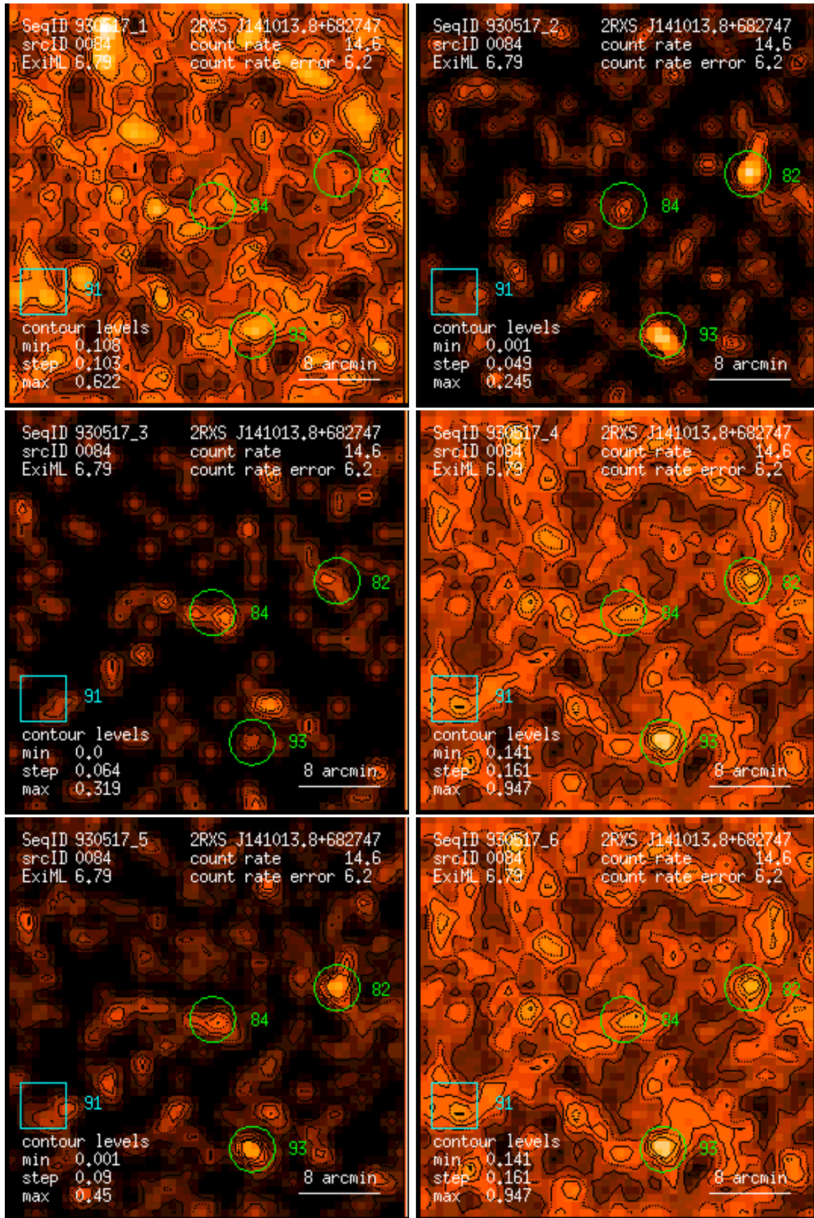
Figure 84: RASS 930517: detection 0084: band rate images, Gaussian filter: (1) PSPC channels 11 – 41, (2) 52 – 90, (3) 91 – 201, (4) 11 – 235, (5) 52 – 201, (6) 11 – 201. Broad band rates in counts/ks. Band rate contour levels in counts/ks/arcmin 2 .
