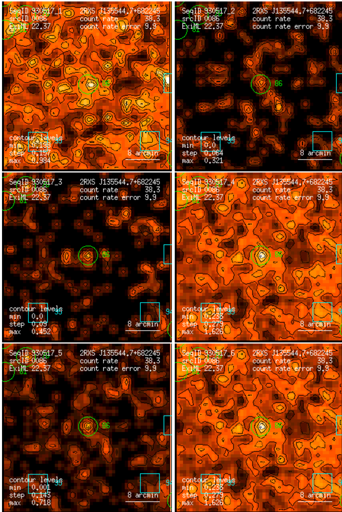
Figure 86: RASS 930517: detection 0086: band rate images, Gaussian filter: (1) PSPC channels 11 – 41, (2) 52 – 90, (3) 91 – 201, (4) 11 – 235, (5) 52 – 201, (6) 11 – 201. Broad band rates in counts/ks. Band rate contour levels in counts/ks/arcmin 2 .
