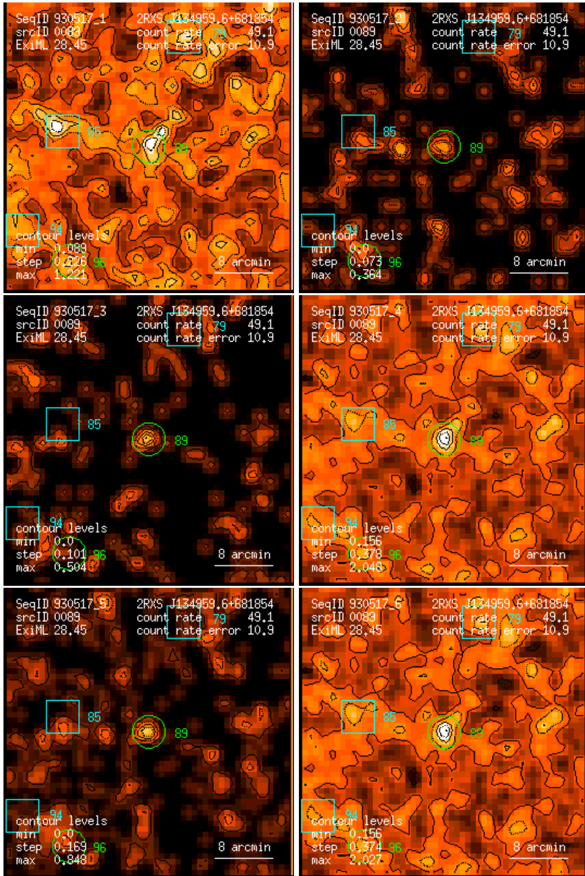
Figure 89: RASS 930517: detection 0089: band rate images, Gaussian filter: (1) PSPC channels 11 – 41, (2) 52 – 90, (3) 91 – 201, (4) 11 – 235, (5) 52 – 201, (6) 11 – 201. Broad band rates in counts/ks. Band rate contour levels in counts/ks/arcmin 2 .
