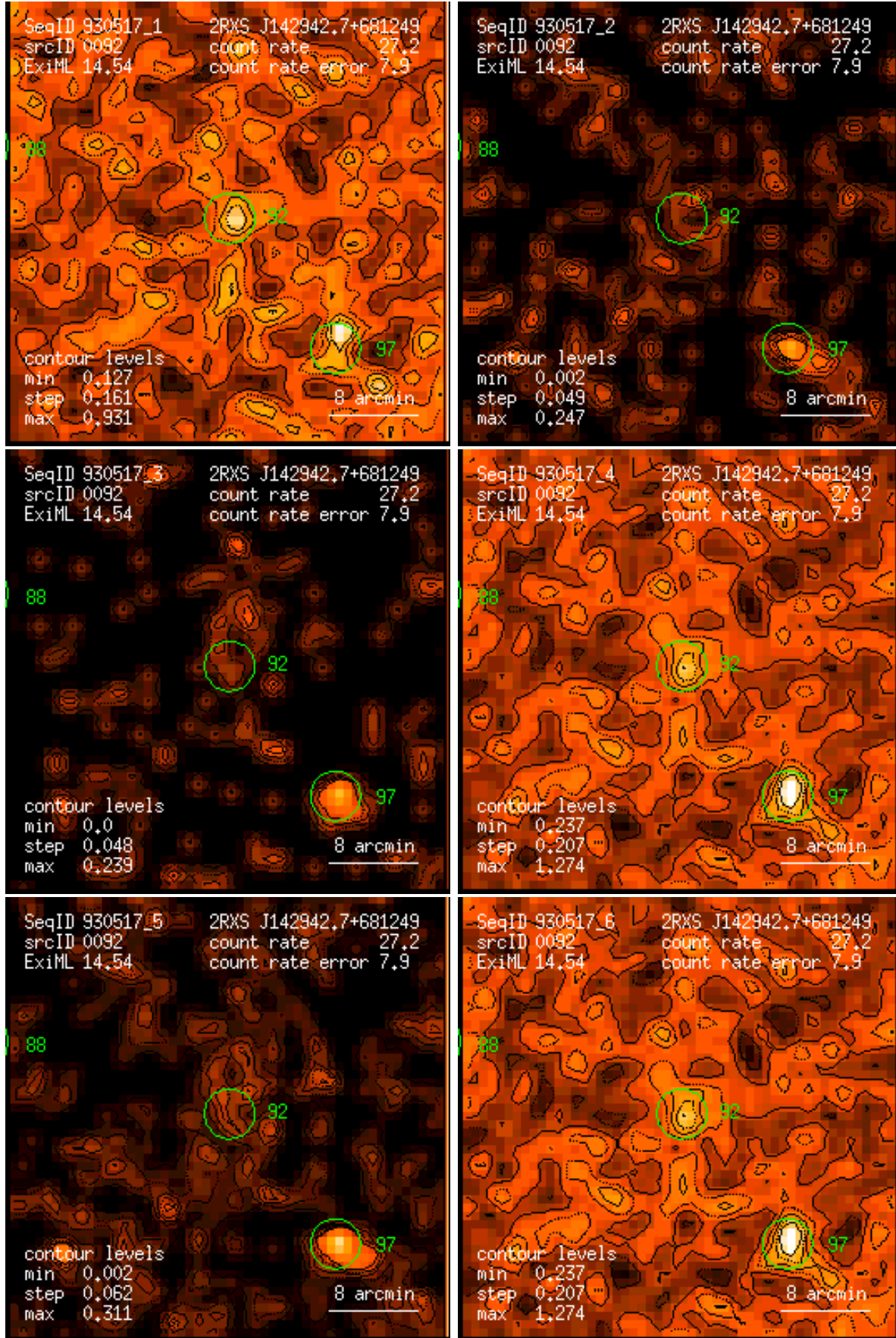
Figure 92: RASS 930517: detection 0092: band rate images, Gaussian filter: (1) PSPC channels 11 – 41, (2) 52 – 90, (3) 91 – 201, (4) 11 – 235, (5) 52 – 201, (6) 11 – 201. Broad band rates in counts/ks. Band rate contour levels in counts/ks/arcmin 2 .
