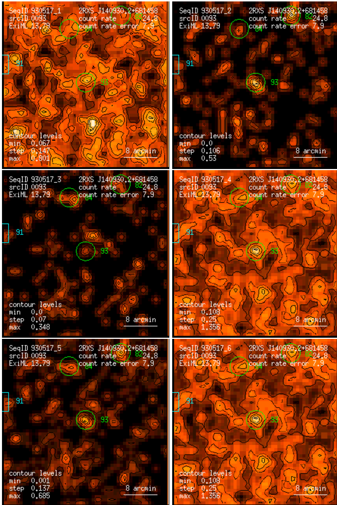
Figure 93: RASS 930517: detection 0093: band rate images, Gaussian filter: (1) PSPC channels 11 – 41, (2) 52 – 90, (3) 91 – 201, (4) 11 – 235, (5) 52 – 201, (6) 11 – 201. Broad band rates in counts/ks. Band rate contour levels in counts/ks/arcmin 2 .
