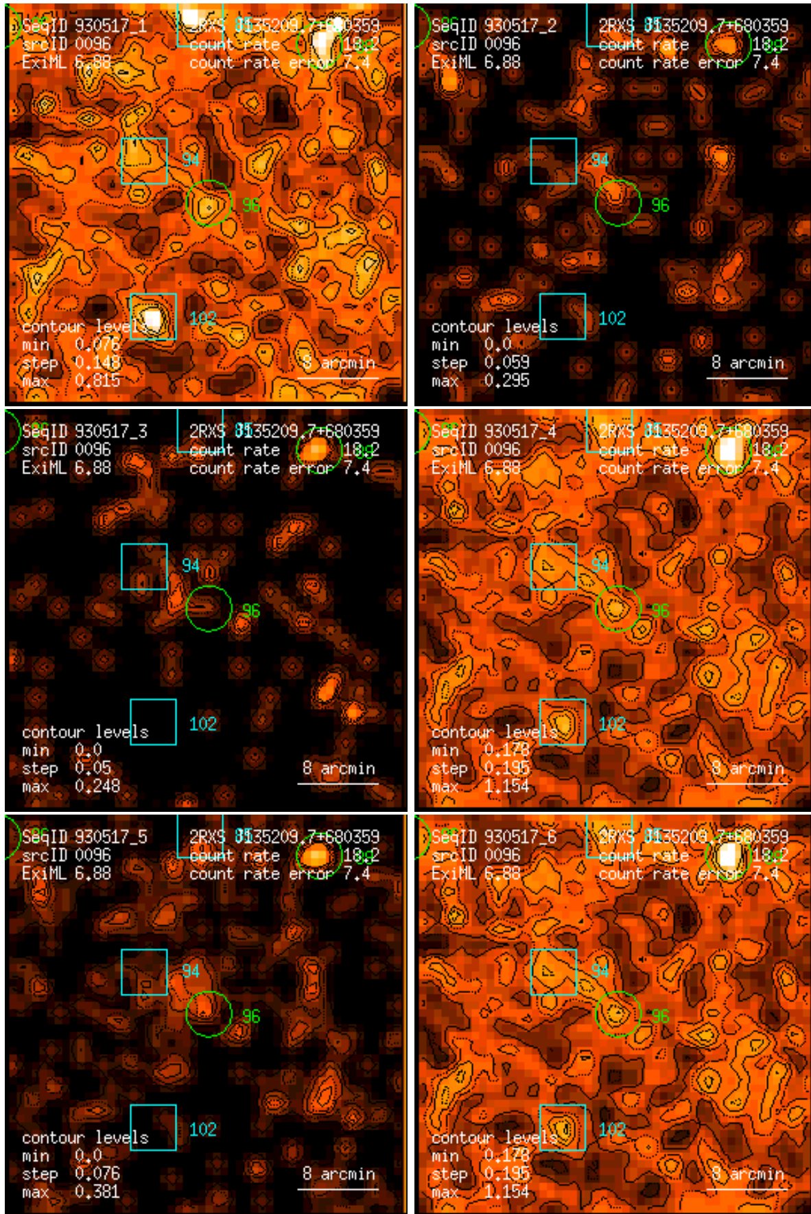
Figure 96: RASS 930517: detection 0096: band rate images, Gaussian filter: (1) PSPC channels 11 – 41, (2) 52 – 90, (3) 91 – 201, (4) 11 – 235, (5) 52 – 201, (6) 11 – 201. Broad band rates in counts/ks. Band rate contour levels in counts/ks/arcmin 2 .
