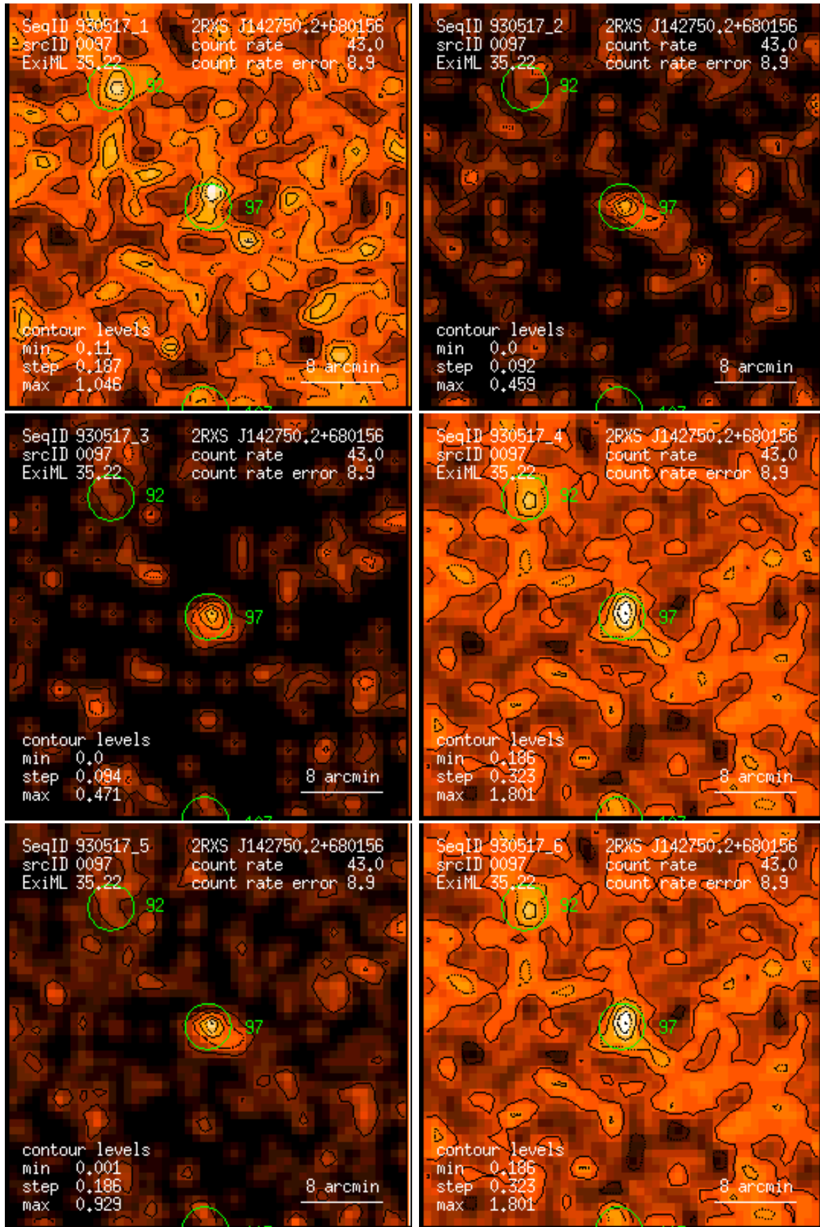
Figure 97: RASS 930517: detection 0097: band rate images, Gaussian filter: (1) PSPC channels 11 – 41, (2) 52 – 90, (3) 91 – 201, (4) 11 – 235, (5) 52 – 201, (6) 11 – 201. Broad band rates in counts/ks. Band rate contour levels in counts/ks/arcmin 2 .
