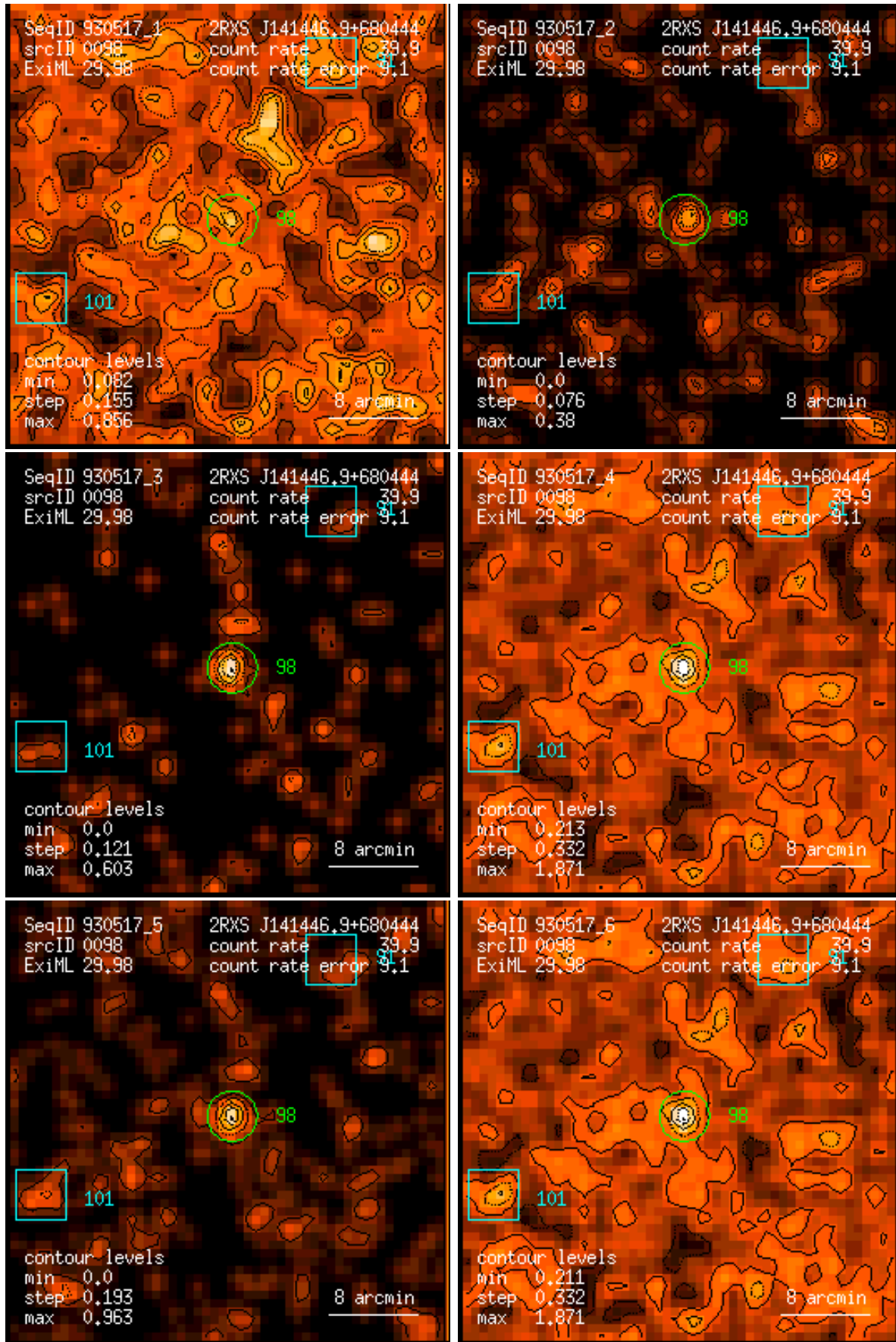
Figure 98: RASS 930517: detection 0098: band rate images, Gaussian filter: (1) PSPC channels 11 – 41, (2) 52 – 90, (3) 91 – 201, (4) 11 – 235, (5) 52 – 201, (6) 11 – 201. Broad band rates in counts/ks. Band rate contour levels in counts/ks/arcmin 2 .
