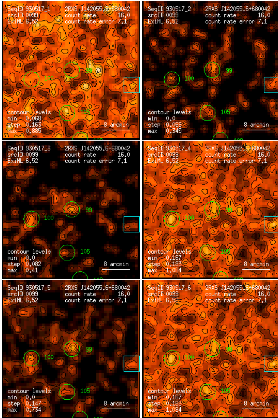
Figure 99: RASS 930517: detection 0099: band rate images, Gaussian filter: (1) PSPC channels 11 – 41, (2) 52 – 90, (3) 91 – 201, (4) 11 – 235, (5) 52 – 201, (6) 11 – 201. Broad band rates in counts/ks. Band rate contour levels in counts/ks/arcmin 2 .
