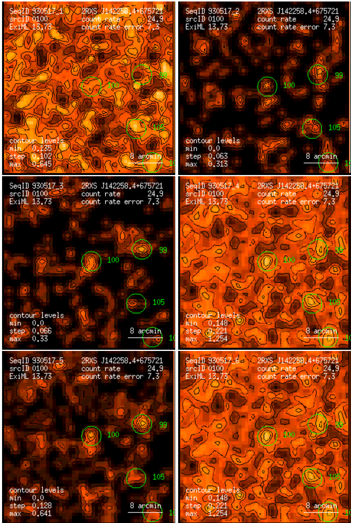
Figure 100: RASS 930517: detection 0100: band rate images, Gaussian filter: (1) PSPC channels 11 – 41, (2) 52 – 90, (3) 91 – 201, (4) 11 – 235, (5) 52 – 201, (6) 11 – 201. Broad band rates in counts/ks. Band rate contour levels in counts/ks/arcmin 2 .
