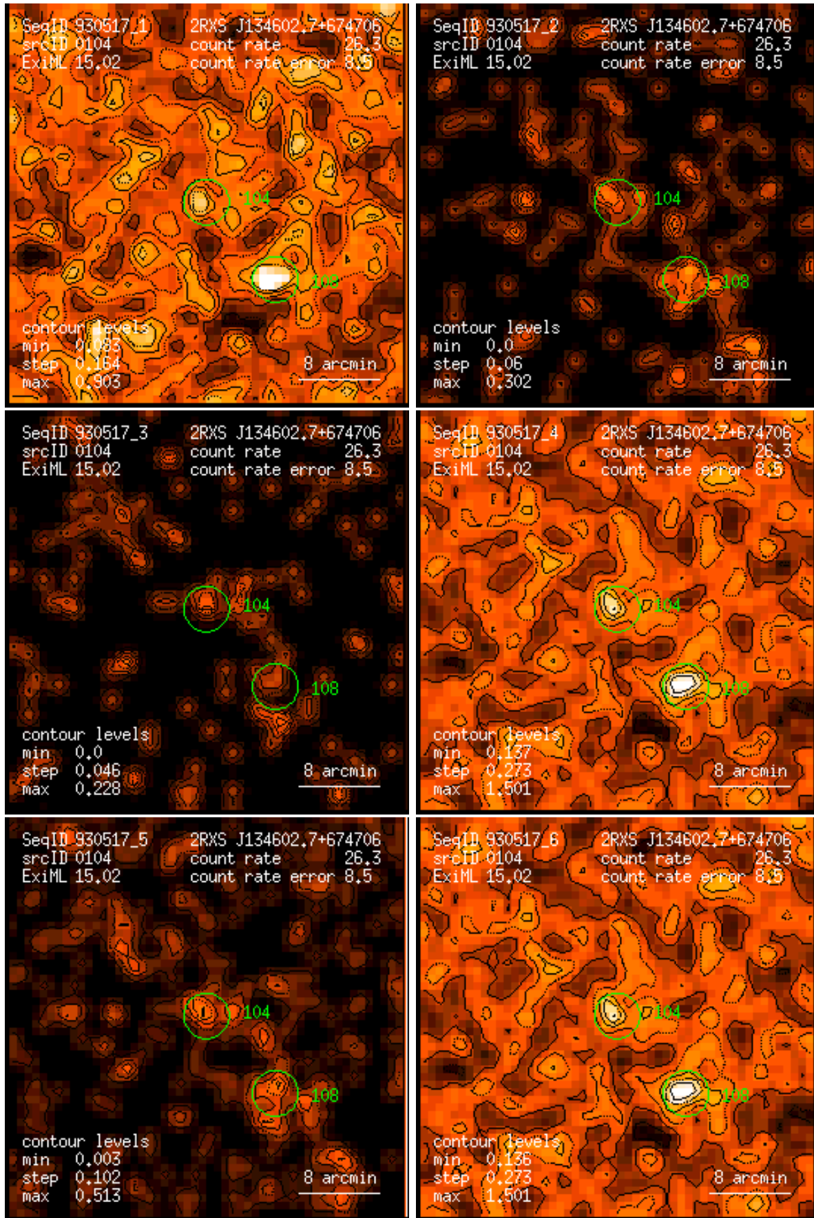
Figure 104: RASS 930517: detection 0104: band rate images, Gaussian filter: (1) PSPC channels 11 – 41, (2) 52 – 90, (3) 91 – 201, (4) 11 – 235, (5) 52 – 201, (6) 11 – 201. Broad band rates in counts/ks. Band rate contour levels in counts/ks/arcmin 2 .
